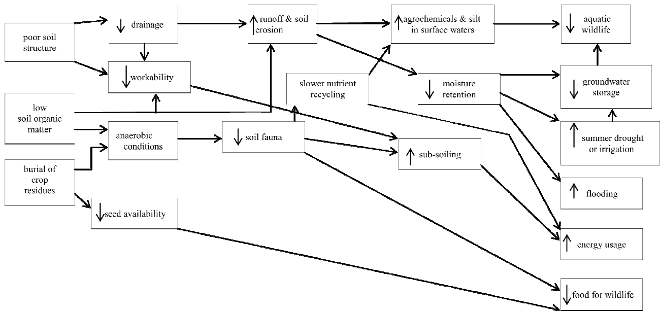
Fig. 2. Processes through which degraded soils affect the environment [20]
