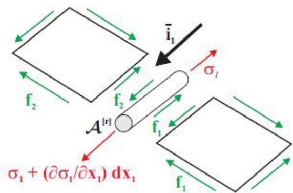
Fig. 8. Stringer sheet idealization of wing structure (Bauchau, 2018)
