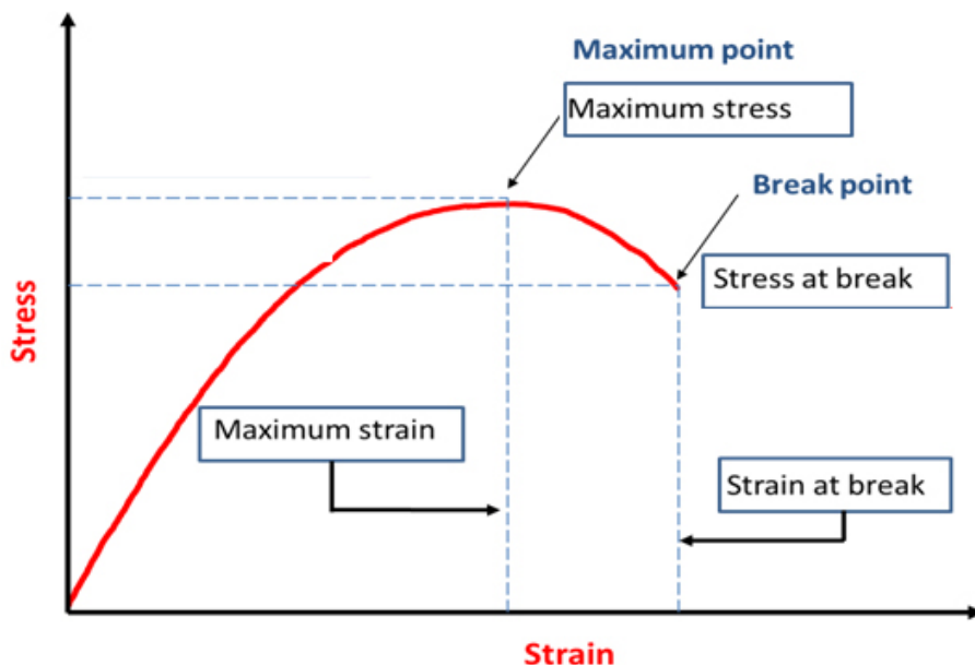
Figure 2. Typical (stress-strain) curve for composite propellants
