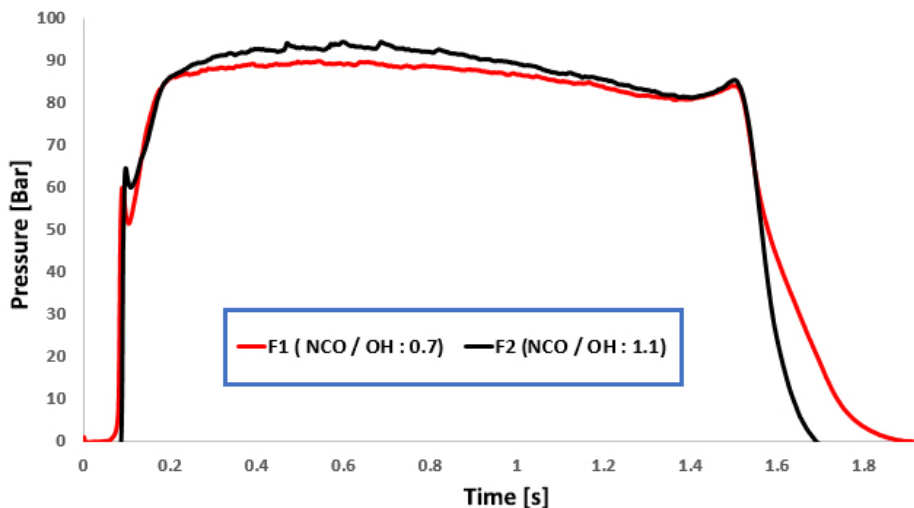
Figure 9. Influence of curing ratio on the pressure-time curves
