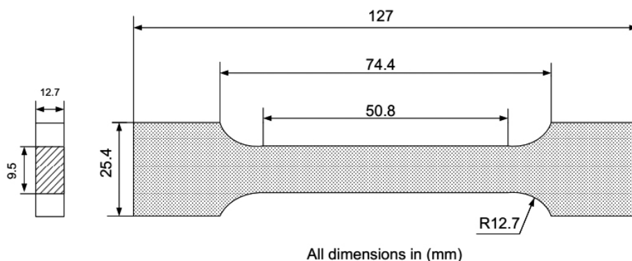
Figure 3. JANNAF specimen for mechanical testing [21]
