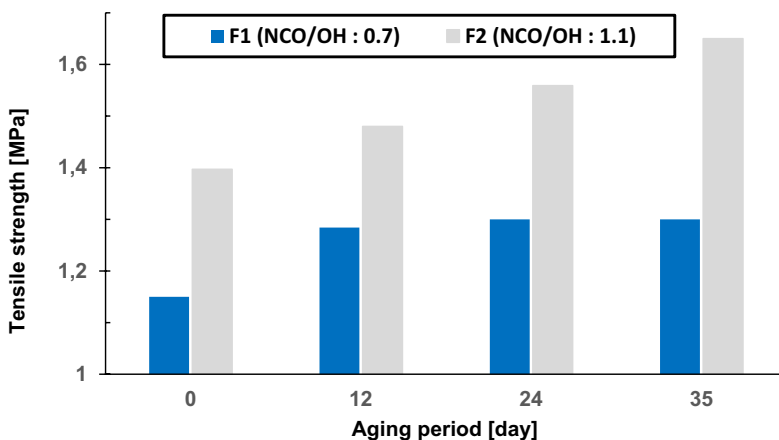
Figure 6. Variation of tensile strength with ageing
