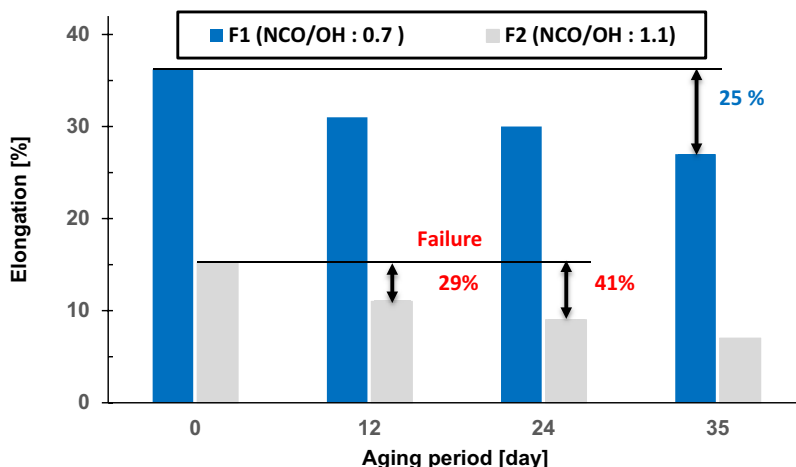
Figure 7. Variation of strain value with ageing
