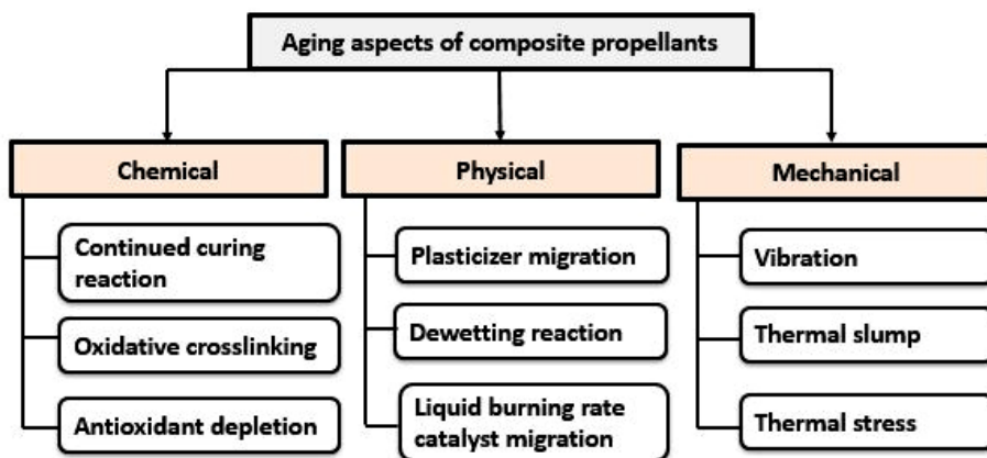
Figure 1. Main ageing aspects of composite propellants
