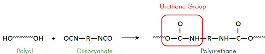
Scheme 1. Curing reaction of a polyol pre-polymer with a di-isocyanate
