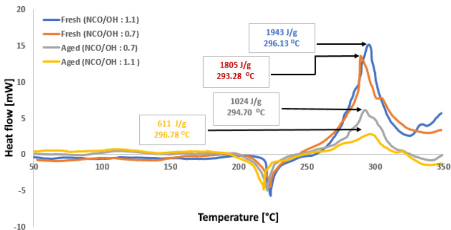
Figure 8. DSC thermograms of fresh and aged formulations after 35 days at 80 °C
