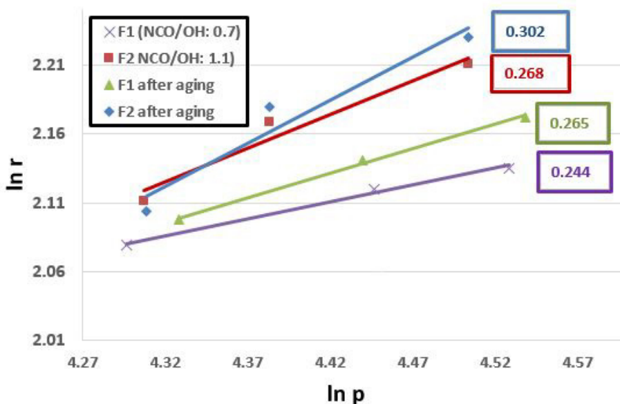
Figure 10. Influence of curing ratio on the pressure exponent n with ageing time
