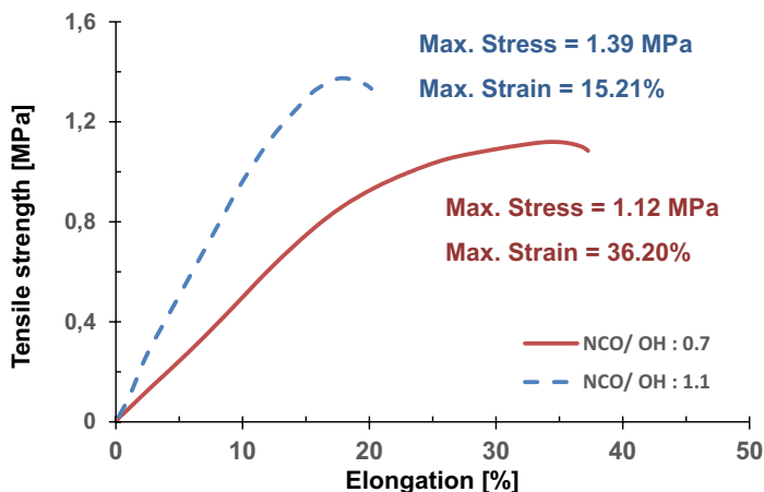
Figure 5. Influence of the curing ratio on the mechanical characteristics of the composite propellant
