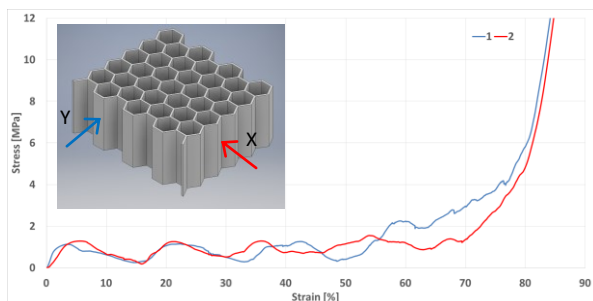
Fig. 5. Stress-strain curves of the cast honeycomb specimens with two orientation of honeycomb channels to load direction
