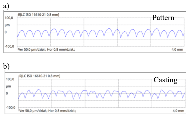
Fig. 2. Surface linear profiles for pattern made by Fused Deposition Modeling (a) and aluminium casting reproduced from polymer pattern (b)
