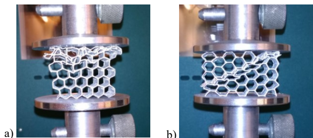
Fig. 4. View of compression tests at two orientation of honeycomb 1 (a) and 2 (b) which results are presented in Fig.3
