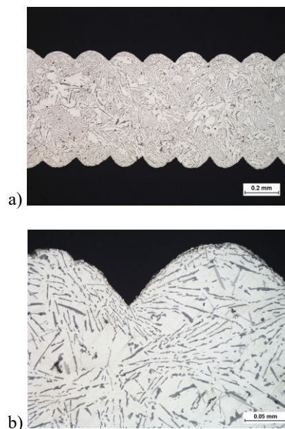
Fig. 3. Microstructure of single wall of aluminium alloy honeycomb element (a), surface of casting with topography after 3D printing pattern (b)
