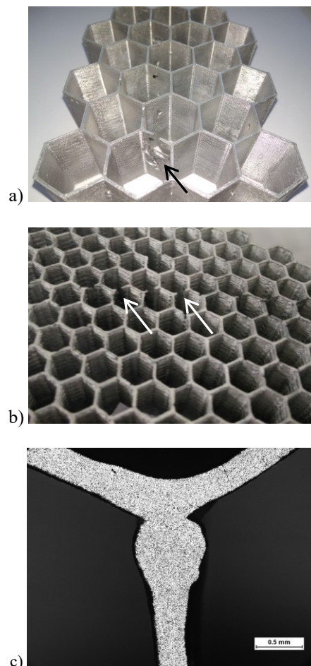
Fig. 1. Perforated walls of incorrect cast honeycomb (a, b), the connection of the three walls (c)
