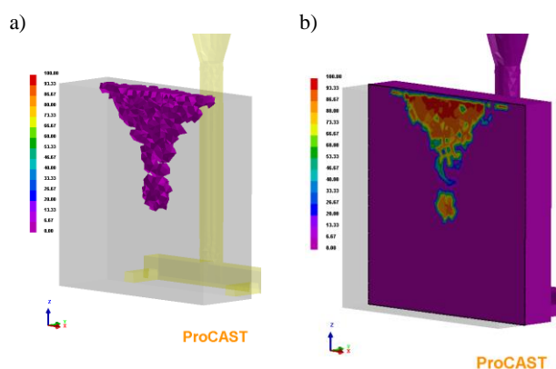
Fig. 4. Shrinkage defects in an inoculated cast iron casting, chemical composition No. 2: a) area of occurrence of shrinkage defects over 1% vol.; b) a cross-section through the center of the plate
