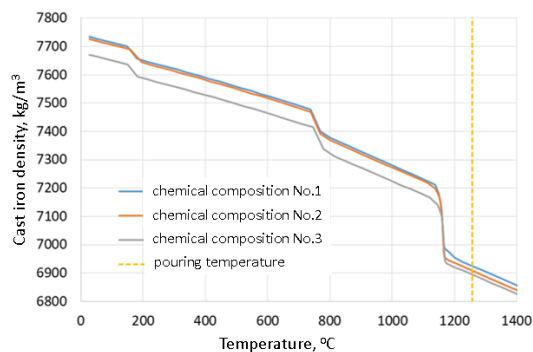
Fig. 2. Change of cast iron density with temperature change (results of calculations for the state of thermodynamic equilibrium, made using the CompuTherm Database)
