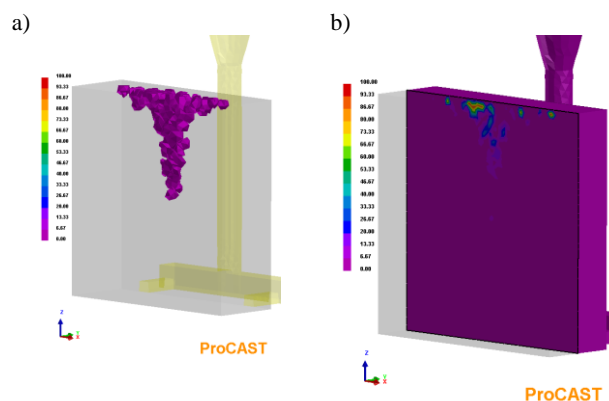
Fig. 5. Shrinkage defects in an inoculated cast iron casting, chemical composition No. 3: a) area of occurrence of shrinkage defects over 1% vol.; b) a cross-section through the center of the plate
