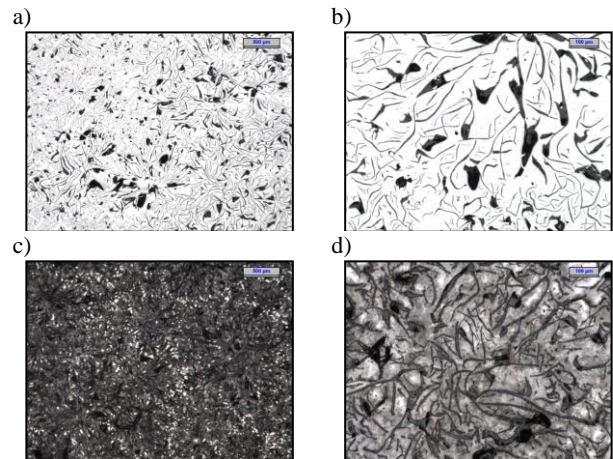
Fig. 7. The microstructure of cast iron after Zircinoc inoculation: non etched - a,b); etched: Stead's reagent - c), nital - d); magnification: 25x - a,c); 100x - b,d)
