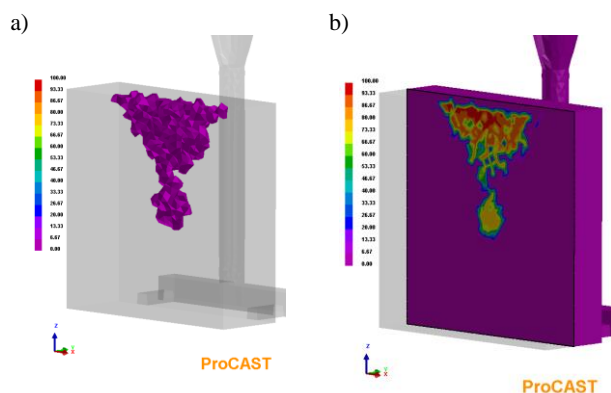
Fig. 3. Shrinkage defects in an inoculated cast iron casting, chemical composition No. 1: a) area of occurrence of shrinkage defects over 1% vol.; b) a cross-section through the center of the plate
