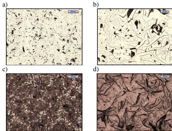
Fig. 6. The microstructure of cast iron after Superseed inoculation: non etched - a,b); etched: Stead's reagent - c), nital - d); magnification: 25x - a,c); 100x - b,d)
