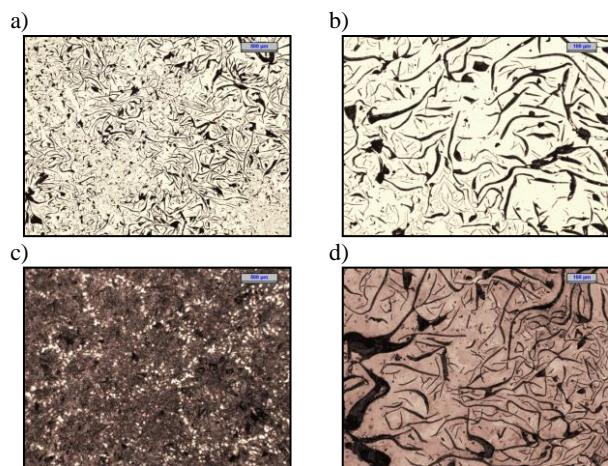
Fig. 8. The microstructure of cast iron after Inolate inoculation: non etched - a,b); etched: Stead's reagent - c), nital - d); magnification: 25x - a,c); 100x - b,d)
