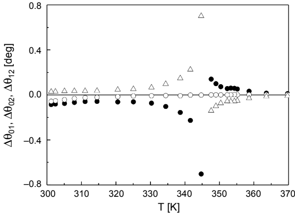
Fig. 1. Temperature dependences of differences among the characteristic azimuthal angles \Delta\theta_{01} ( \bullet ), \Delta\theta_{02} ( \circ ), \Delta\theta_{12} ( \triangle ) for the CGG crystals as measured for one of the orientations of specimen in the PSA system at 780 nm.
