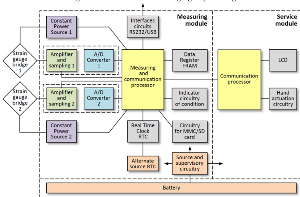
Fig. 5. Accumulating unit
