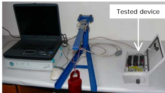
Fig. 6. Beam of constant strength connected to the computer and the tested device
