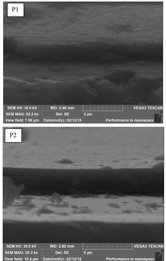
Fig. 3. Cross-section of \text{TiO}_2 thin films deposited on silicon substrates
