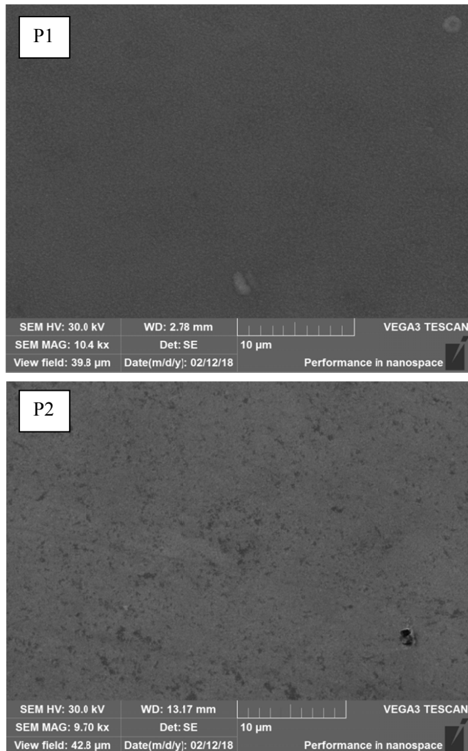
Fig. 2. SEM images of pure \text{Cu}_2\text{O} thin films deposited on silicon substrates
