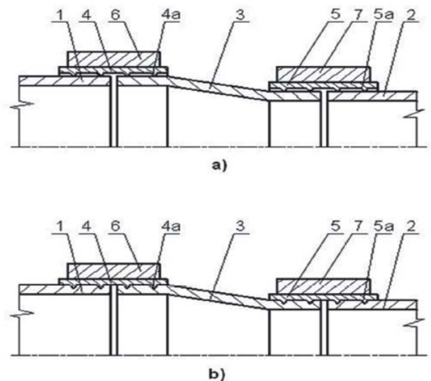
Fig. 11. Diameter-reducing member joint using heat-shrinkable sleeves made of the SMA: a) pipe joint before thermal deformation; b) pipe joint after thermal deformation. 1 and 2 – ends of pipes, 3 – diameter-reducing pipe joint, 4 – large-diameter liner, 5 – small-diameter liner, 4a and 5a – projections and 6 and 7 – heat-shrinkable sleeves made of SMA heating element
