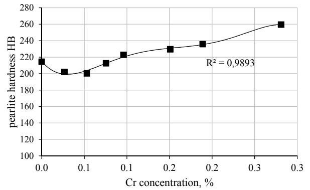
Fig. 9. Pearlite microhardness vs chromium concentration in vermicular graphite cast iron
