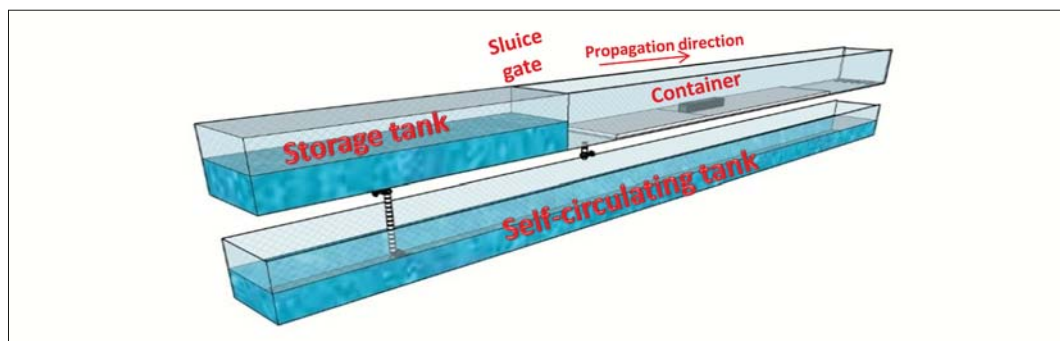
Fig. 2 Stereogram of the test flume and set-up of the model
