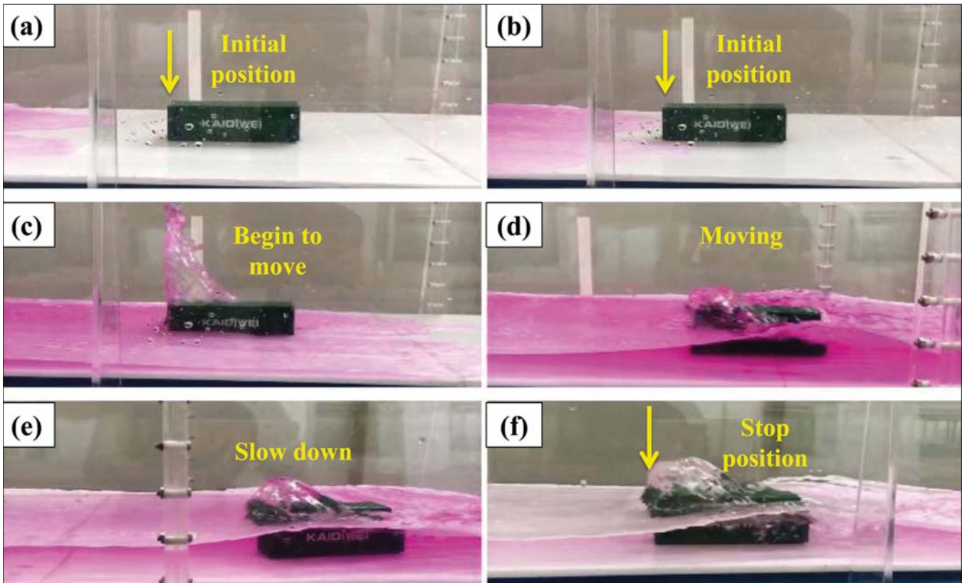
Fig. 4. Process of tsunami waves impacting container model
