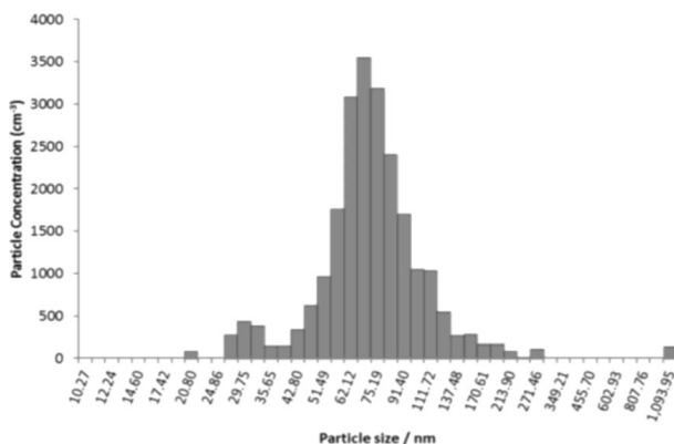
Fig. 2. Sizes of particles produced during the FDM process [17].
