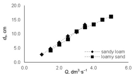
Fig. 7. Scour depth ( d_s ) and discharge ( Q ) for both material in 0.5 \text{ cm} opening height; source: own study
