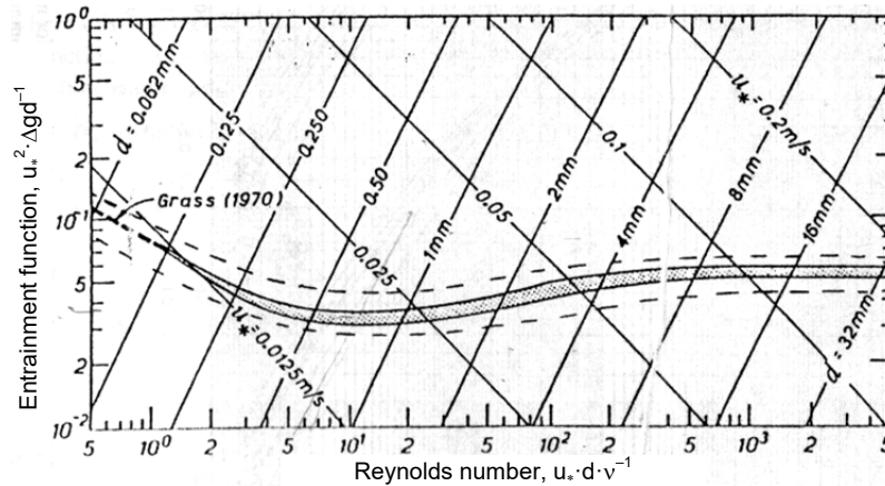
Fig. 1. Shields' curve: u_* = critical velocity, \rho_s = sediment density, d = diameter size of sediment, \nu = kinematics viscosity; source: BREUSERS, RAUDKIVI [1991]
