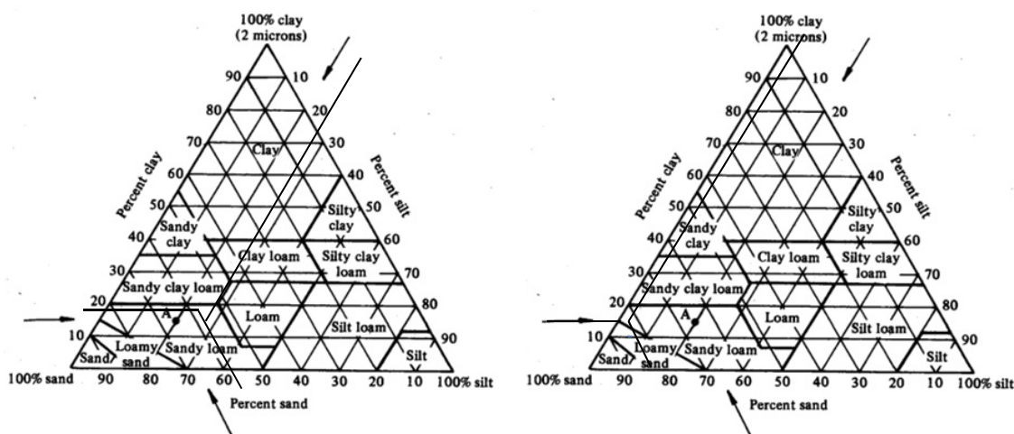
Fig. 4. Classification of sand clay material: a) sandy loam, b) loamy sand; source: FOTH [1984]
