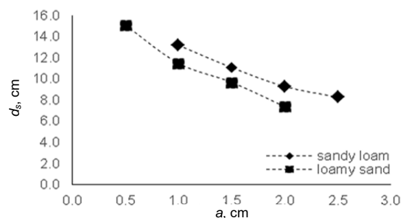
Fig. 6. Scour depth ( d_s ) and height of opening gate ( a ) for both bed material; source: own study
