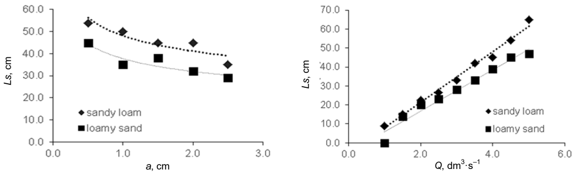
Fig. 10. Length of scour depth and height of opening gate for both bed material; source: own study
