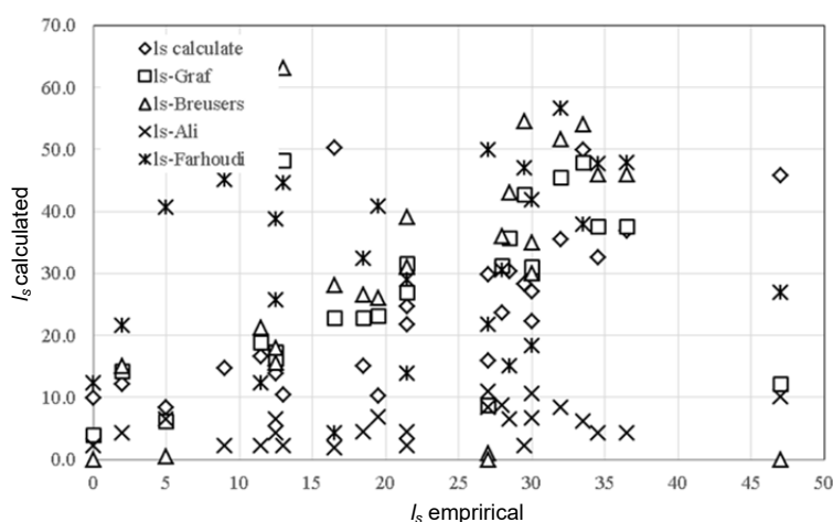
Fig. 13. Comparison between calculated depth of scour ( l_s ) and experimental given by earlier researcher; source: own study
