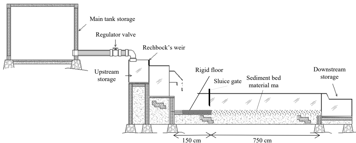
Fig. 3. Experimental setup for scour hole at open channel flume; source: own elaboration
