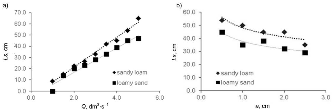
Fig. 12. Coefficients correlation discharge Q (a) and a (b) to scour length ( L_s ); source: own study
