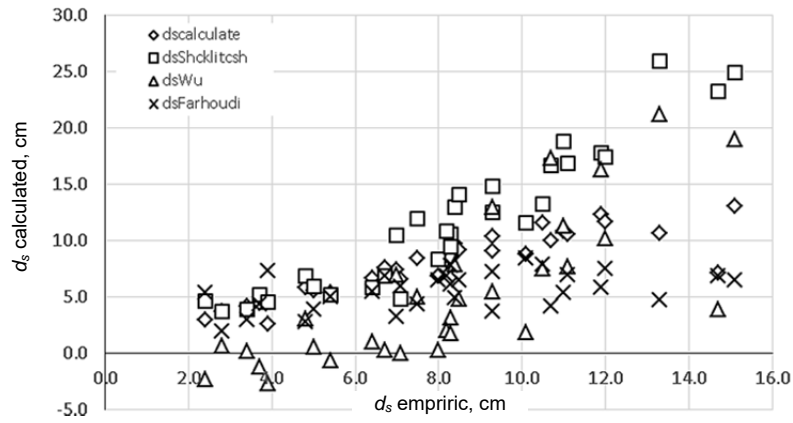
Fig. 8. Comparison between calculated depth of scour ( d_s ) and experimental given by earlier researcher; source: own study
