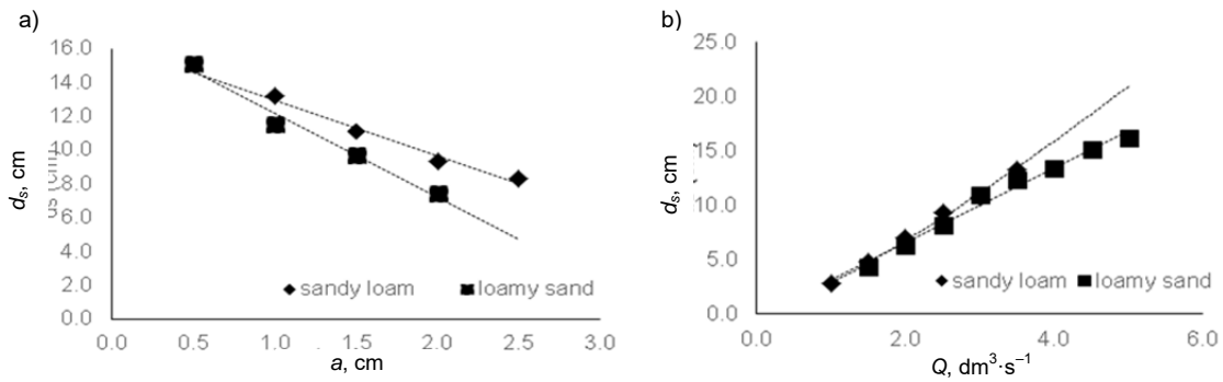
Fig. 9. The coefficients correlation a (a) and Q (b) to scour depth ( d_s ); source: own study
