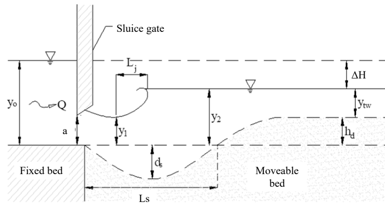
Fig. 2. Parameters of the calculation of scour characteristics; L_j = hydraulic jump, L_s = length of scour, y_0, y_1, y_2, y_{tw}, h_D, d_s, Q, a as under the Eq. (1); source: own elaboration
