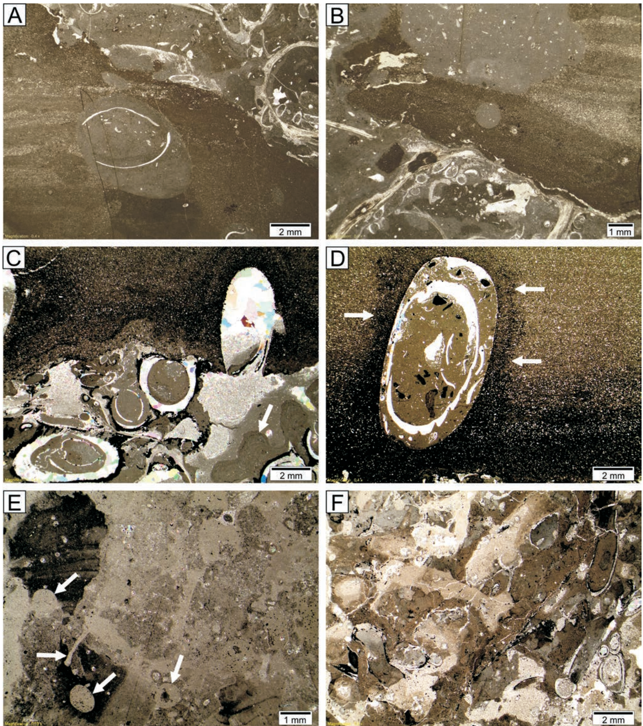
Fig. 8. Microfacies observed in layer with bored and encrusted HCs from Sobków Quarry and N71P and 21P wells. A. In the lower part of the photograph, pyritized HC is visible consist of bored thin-laminated microbioclastic-peloidal calcisiltite. In the upper part of the photograph, bioclastic wackestone with serpulids and bivalves is observed (Sobków Quarry). B. In the central part of the photograph, strongly abraded HC built of thin-laminated calcisiltite. In the lower part of the photograph, bioclastic wackestone with serpulids and bivalves, occurs (Sobków Quarry). C. In the lower part of the photograph, serpulid colony bored by bivalves is observed. Microbialites (arrow) are visible on the serpulids. In the upper part of the photograph, calcisiltite with bivalve boring is visible, around the boring aureole of pyritized sediments is present (N71P well). D. Bored HC built of thin-laminated packstone-wackestone with the bivalve boring Gastrochaenolites , in the boring shells are seen representing a few generations of bivalves, around the boring aureole of pyritized sediments is present (arrows) (N71P well). E. Strongly bioturbated wackestone, on the left small, abraded, angular, fine-laminated HCs are seen with Trypanites and Gastrochaenolites (arrows) (21P well). F. Fragment of strongly bioeroded HC with serpulids colony (21P well).
