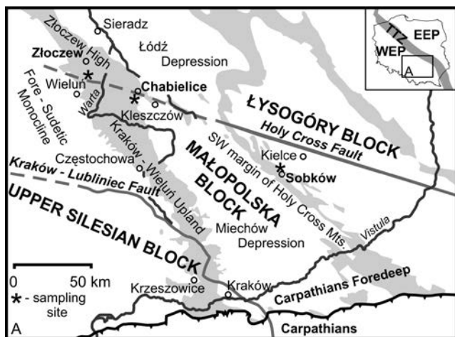
Fig. 1. Location map of the study areas with Upper Jurassic outcrops and sub-Cenozoic Upper Jurassic subcrops (grey) in southern and Central Poland (after Pożaryski et al. , 1979; modified and simplified). Names in italics indicate location of main tectonic structures in the Palaeozoic basement (after Buła and Habryn, 2011; Żelaźniewicz et al. , 2011). TTZ – Teisseyre-Tornquist Zone, EEP – East European Platform, WEP – West European Platform.
