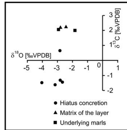
Fig. 10. Carbon and oxygen isotopic data for hiatus concretion, matrix of layer and underlying marls from N71P well.
