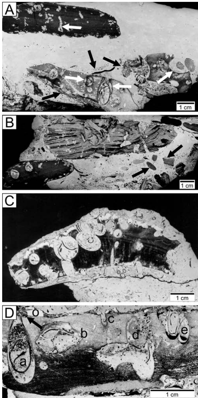
Fig. 3. Bored and encrusted HCs from the Sobków Quarry (polished slabs, new reprints of the archival material from Chudzikiewicz and Wieczorek, 1985). A. Upper part: HC showing dark, fine lamination; lower part: two HCs with biogenic layer composed of oysters and serpulids (black arrows). In the HCs, numerous borings Trypanites and Gastrochaenolites are visible. Some of the borings are strongly truncated (white arrows). Reprint of plate I/2. B. Bored HCs showing differences in lamination; on the right, numerous, small, angular HCs are seen (arrows). Matrix of the layer consists of small HCs, bioclasts, oysters and oncoids). Reprint of plate II/1. C. Trichites shell with biogenic layer on the upper part, some of the borings cut through the biogenic layer, white patches on the shell represent silicified areas; reprint of plate VII/6. D. Enlarged fragment of the HC: (a) bivalve boring Gastrochaenolites with fine-detrital internal sediment and bivalve shell, (o) encrusting oyster bored by bivalve (black arrow), (b) Gastrochaenolites with lower parts encrusted by serpulids (c) Trypanites , (d) cavity formed by a few generations of the bivalve boring Gastrochaenolites , (e) a few generations of Gastrochaenolites with geopetal infillings; reprint of plate II/3.
