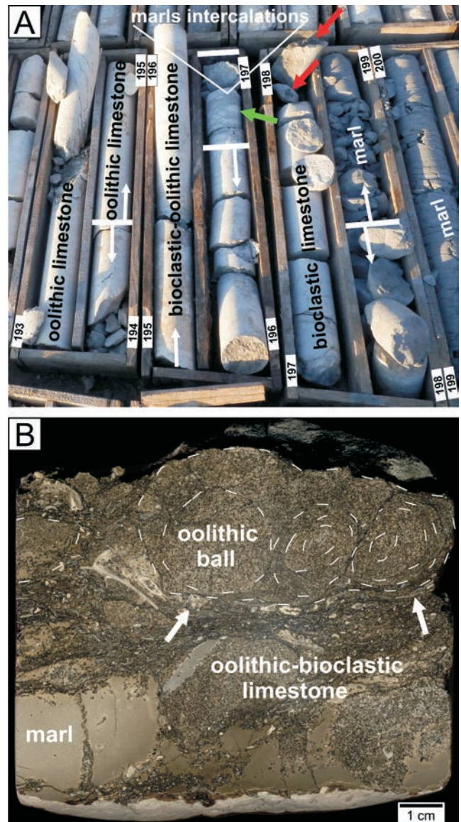
Fig. 4. Sedimentary sequence of the N71P well with localization of the HCs and oolitic balls. A. Fragment of drill core from N71P well (Łódź Depression) with marked lithological horizons presented in Fig. 2 and depth intervals. Red arrows point to position of bored and encrusted HCs within sedimentary sequence; green arrow indicates position of oolitic balls. B. Polished slab; in the lower part marls, in the upper part oolitic balls (see Radwański, 1960), white arrows indicate encrustations on the balls. This succession documents the beginning of the development of the Lower Kimmeridgian oolitic shallow platform in the Łódź Depression.
