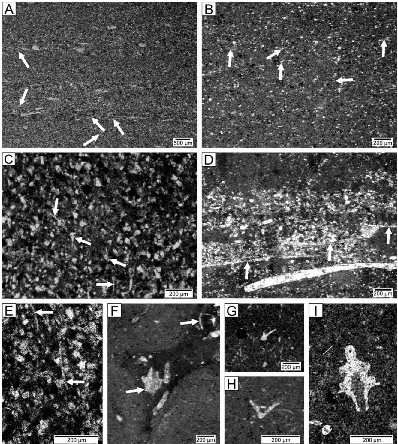
Fig. 9. Microfacies of HCs from Sobków Quarry and N71P and 21P wells. A. Microbioclastic peloidal fine laminated calcisiltite; fine-grained packstone-wackestone with peloids, filaments (arrows), echinoderms and bivalves; Sobków Quarry. B. Microbioclastic peloidal wackestone with rare Saccocoma remains (arrows); N71P well. C. Microbioclastic packstone-wackestone calcisiltite with filaments (arrows); Sobków quarry. D. Microbioclastic calcisiltite with filaments (arrows) and bivalve in the lower part which pass into bioclastic wackestone in the upper part; Sobków quarry. E–I. Remains of Saccocoma secundibranchials (E, F – Sobków Quarry; G, H – N71P well; I – 21P well).
