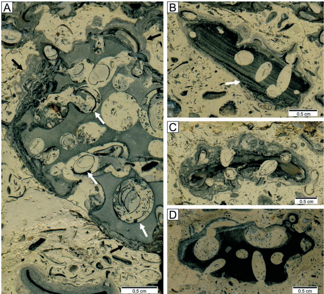
Fig. 7. Details of layer with bored and encrusted HCs from N71P well (for location of A–C see Fig. 6B). A. Silicified HC with numerous bivalve boring Gastrochaenolites ; in borings shells are visible with a few generations of bivalves (white arrows); on the outer surfaces encrustations are seen: bivalves, serpulids and microbialites (black arrows). B. Small, angular, fine-laminated HC, in the lower right part of the HC cross-lamination is visible (white arrow), outer surfaces around the HC consist of well-developed, encrusting biogenic layer with bivalves, serpulids and microbialites, in the central part of the HC numerous Gastrochaenolites are seen. C. Expanded view of strongly bored oncoïd, on bivalve nuclei the organism-bearing microbial envelope grows, truncated by the bivalve boring Gastrochaenolites . D. Small HC with Gastrochaenolites Gastrochaenolites . Some of the borings are strongly abraded; others are filled with micrite and bioclasts, composed of material identical to the enclosing sediment.
