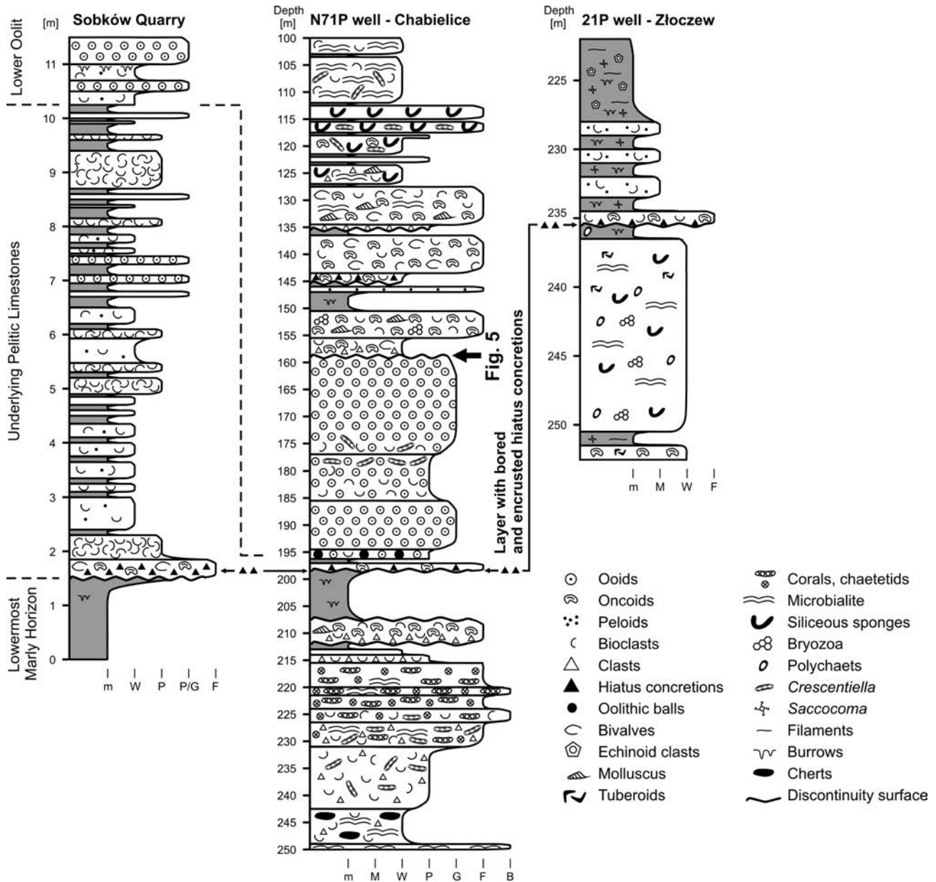
Fig. 2. Examples of lithological columns from the study areas, with positions of the layer with bored and encrusted HCs marked. In the N71P well column, the position of other regional hardgrounds (see Fig. 5; cf. Kaźmierczak and Pszczółkowski, 1968) is marked between the Oolitic and the Oncolithic Limestones horizons. Sobków Quarry – SW margin of the Holy-Cross Mts (after Chudzikiewicz and Wieczorek, 1985; modified), N71P well – Łódź Depression, 21P well – Złoczew High; m – marl, M – mudstone, W – wackestone, F – floatstone, P – packstone, G – grainstone.
