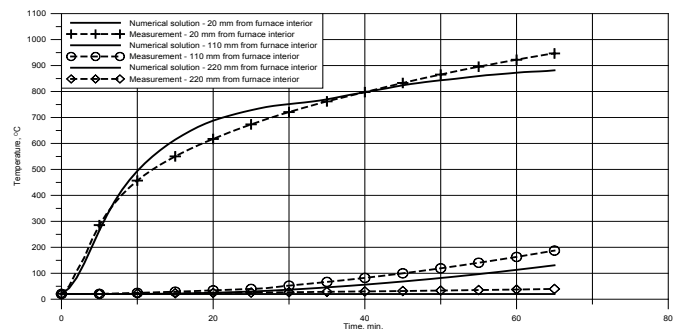
Fig. 6. Comparison of the numerical calculations of the furnace temperature with measurements at the test station
