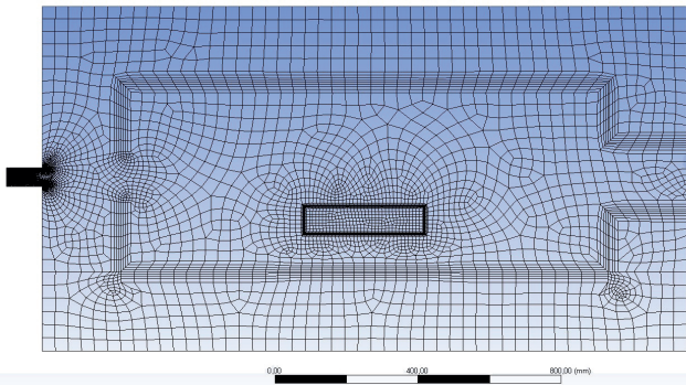
Fig. 2. The geometry and the numerical mesh applied in the laboratory furnace model
