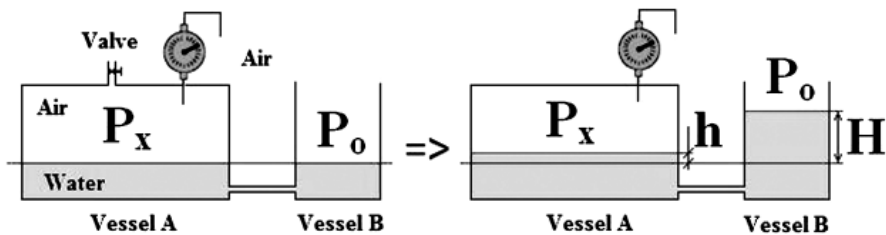
Fig. 2. The scheme presenting the idea of measurement of small values of hydrostatic pressures
