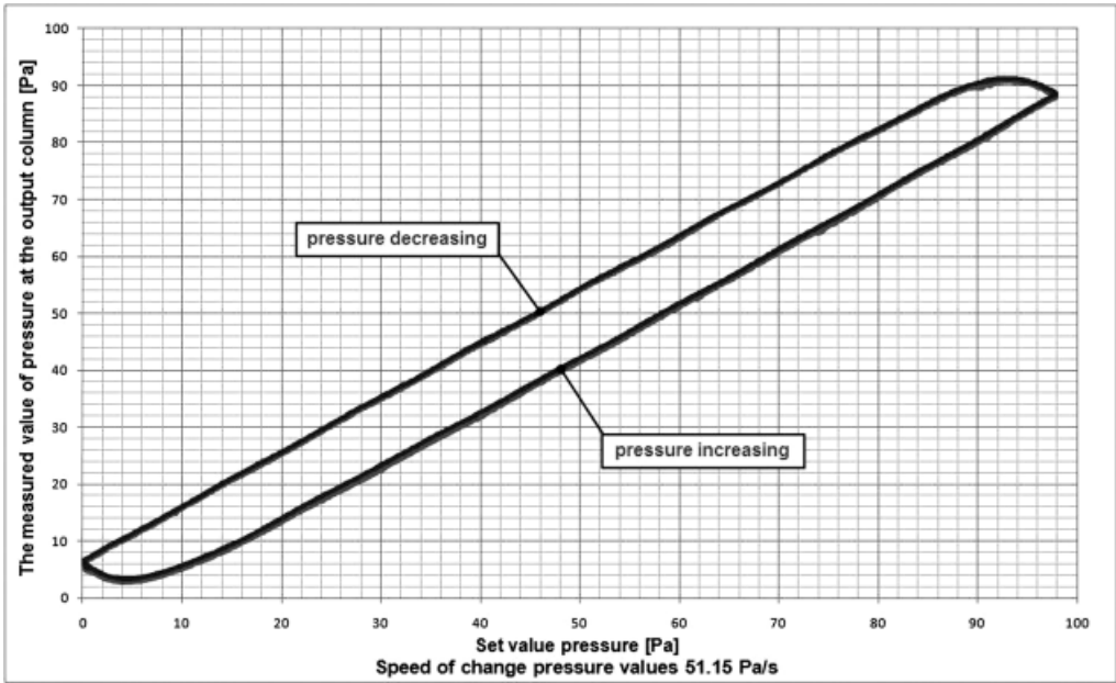
Fig. 5. Hysteresis of measurement of the hydrostatic pressure value for rapid changes of measured value
