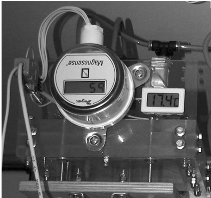
Fig. 4. Gauging tool for small values of hydrostatic pressures
