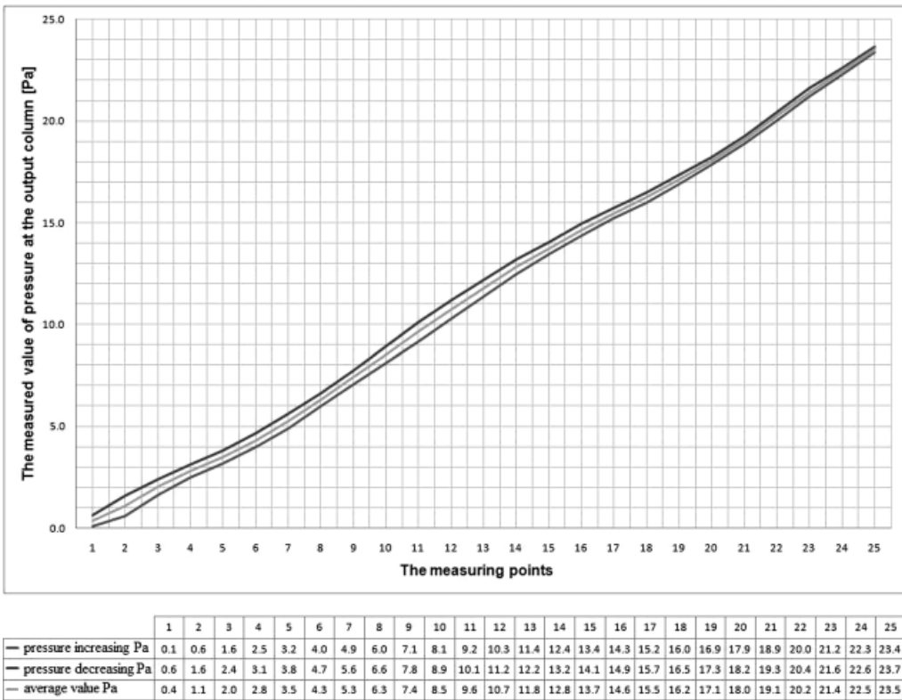
Fig. 8 Influence of atmospheric pressure on measurement process at short times of measurement
