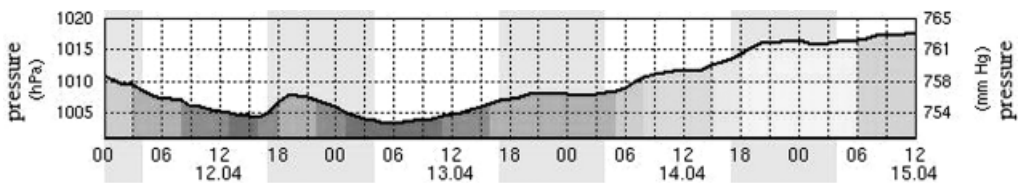
Fig. 3 Pressure reduced to sea level of the city of Cracow. http://new.meteo.pl/
