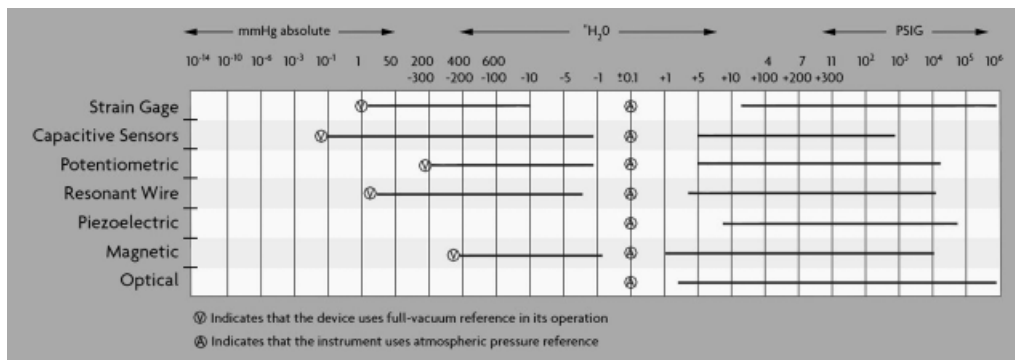
Fig. 1. Diagram showing the range of measured values of pressure for various types of sensors (Raymond, 1997, 1998)
