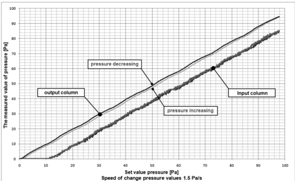
Fig. 6. Hysteresis of measurement of hydrostatic pressure for small changes of measured value
