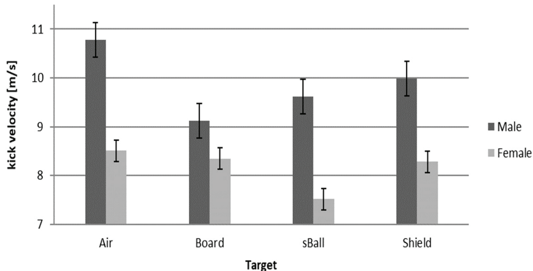
Fig. 3. The joint effect of gender and target on kicking maximum velocity. sBall – small ball (pingpong ball)
