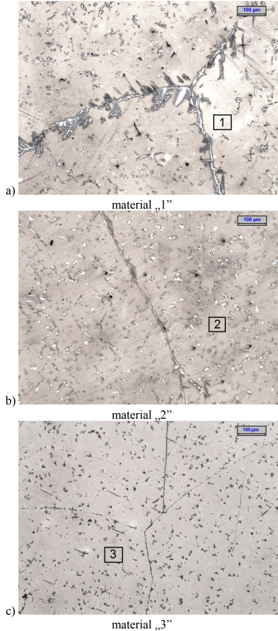
Fig. 2. Microstructure of investigated cast steel (Table 1)
