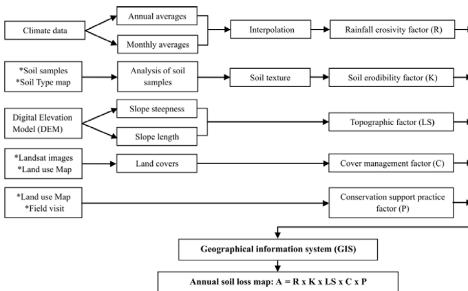
Fig. 5. Flowchart of the GIS based RUSLE methodology; source: own study
