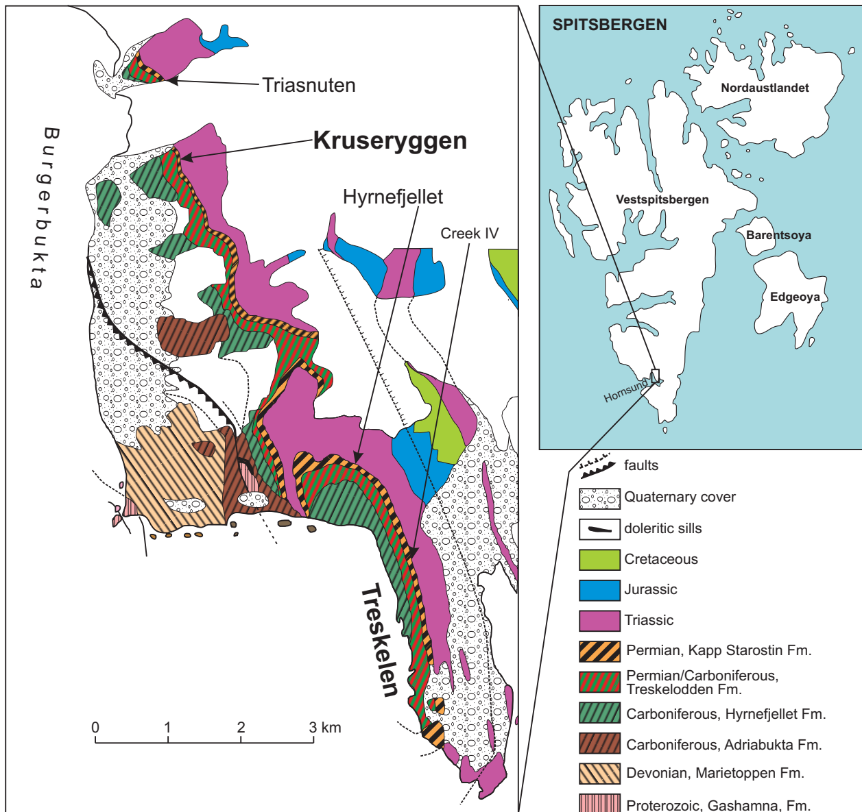
Fig. 1. Geological map of the inner Hornsund area (simplified after Birkenmajer & Fedorowski, 1980).
