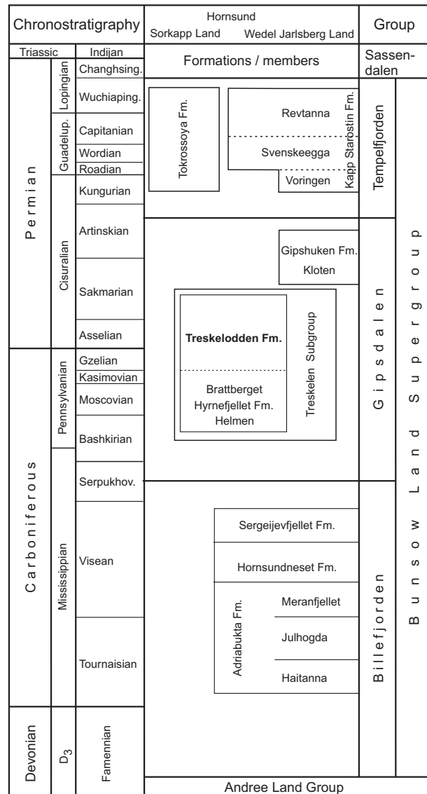
Fig. 2. Lithostratigraphic scheme of the Carboniferous and Permian formations of the Bünsow Land Supergroup recognized in the Hornsund area (simplified after Harland, 1997).
