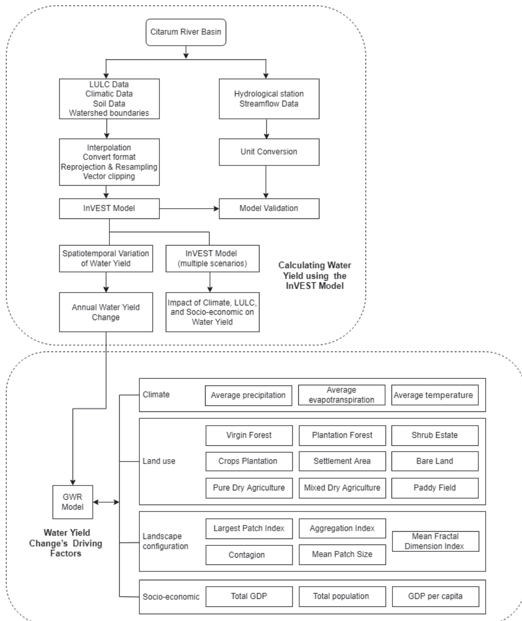
Fig. 2. Research flowchart
