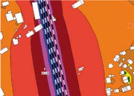
Figure 4. Map L_{day} calculated for a measurement point with the Nordic model [29]. Notes. L_{day} —A-weighted long-term average sound level as defined in Standard No. ISO 1996-2:2007 [37], determined over all day periods of a year.
