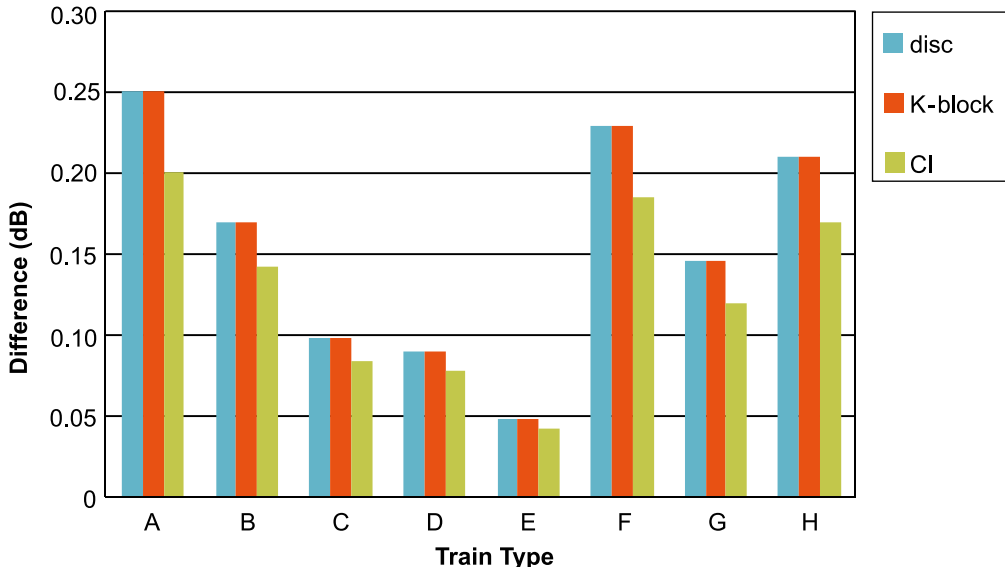
Figure 7. Difference in the equivalent noise level between 1200- and 920-mm wheel diameters for accelerating. Notes. disc—disc-braked vehicles, K-block—K-block braked vehicles, CI—cast-iron block-braked vehicles; K-block braked vehicles, CI—cast-iron block-braked vehicles; A—NS Mat64 EMU (Werkspoor/ Düwag/ Waggonfabrik Talbot, The Netherlands); B—NS 1700 (Alsthom, The Netherlands); C—SNCF BB66400 (Vossloh España, Spain); D—SNCF CC72000 (Alsthom-Atlantique, France); E—RENFE (DLoco, Spain); F—NS6400 (MaK/ABB, Germany); G—TKOJ JT 42CWR (EMD, USA); H—DM90 DMU (Dewag/Talbot/SIG, Germany).
