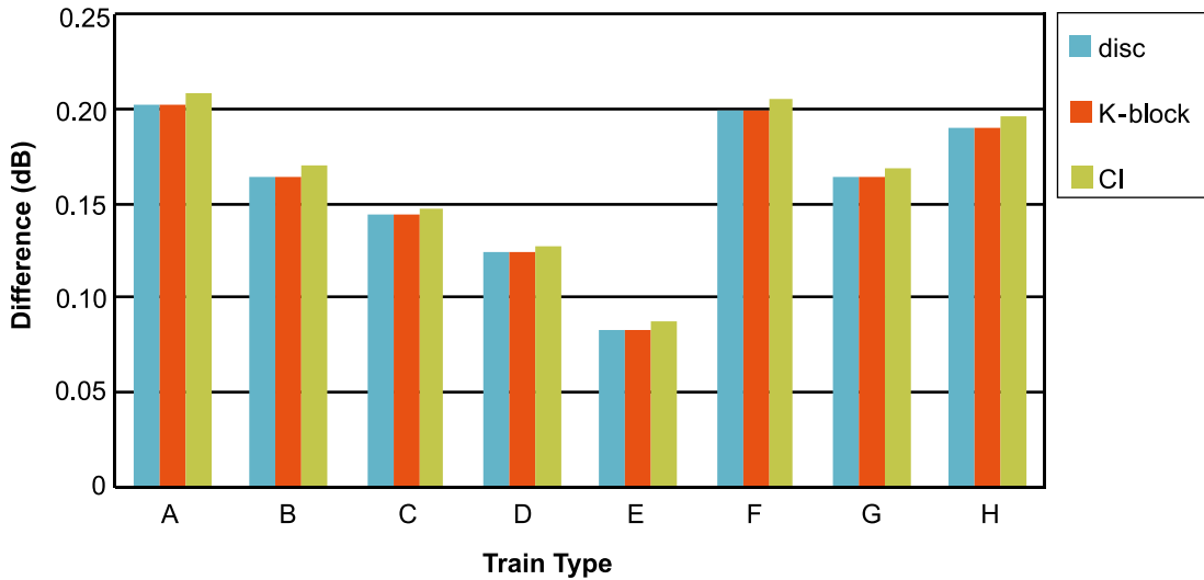
Figure 6. Difference in the equivalent noise level between 920- and 840-mm wheel diameters for constant speed. Notes. disc—disc-braked vehicles, K-block—K-block braked vehicles, CI—cast-iron block-braked vehicles; K-block braked vehicles, CI—cast-iron block-braked vehicles; A—NS Mat64 EMU (Werkspoor/ Düwag/ Waggonfabrik Talbot, The Netherlands); B—NS 1700 (Alsthom, The Netherlands); C—SNCF BB66400 (Vossloh España, Spain); D—SNCF CC72000 (Alsthom-Atlantique, France); E—RENFE (DLoco, Spain); F—NS6400 (MaK/ABB, Germany); G—TKOJ JT 42CWR (EMD, USA); H—DM90 DMU (Duewag/Talbot/SIG, Germany).
