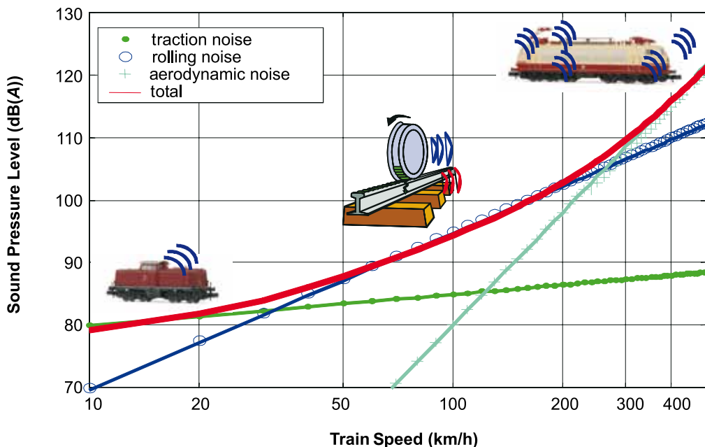
Figure 1. Relative strength and speed dependence of sources of railway noise [3].
