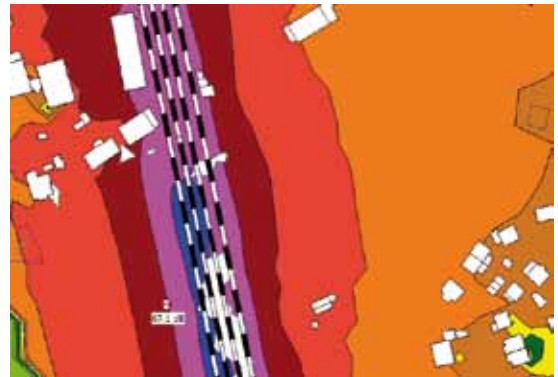
Figure 2. Map L_{day} calculated for a measurement point with Schall 03 [3]. Notes. L_{day} —A-weighted long-term average sound level as defined in Standard No. ISO 1996-2:2007 [37], determined over all day periods of a year.
