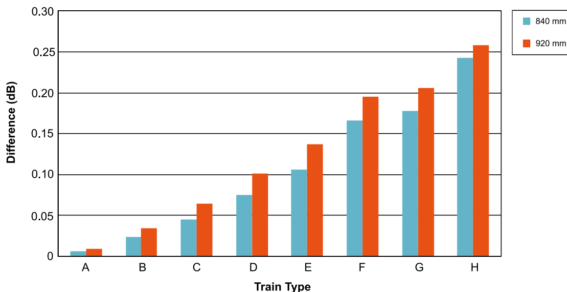
Figure 9. The gap between maximum and minimum noise level differences for CI and K-block brakes with 840- and 920-mm wheel diameters. Notes. K-block braked vehicles, CI—cast-iron block-braked vehicles; A—NS Mat64 EMU (Werkspoor/ Düwag/ Waggonfabrik Talbot, The Netherlands); B—NS 1700 (Alstom, The Netherlands); C—SNCF BB66400 (Vossloh España, Spain); D—SNCF CC72000 (Alstom-Atlantique, France); E—RENFE (DLoco, Spain); F—NS6400 (MaK/ABB, Germany); G—TKOJ JT 42CWR (EMD, USA); H—DM90 DMU (Duewag/Talbot/SIG, Germany).
