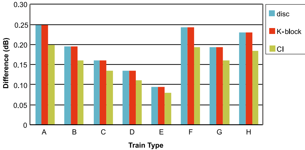
Figure 5. Difference in the equivalent noise level between 1200- and 920-mm wheel diameters for constant speed. Notes. disc—disc-braked vehicles, K-block—K-block braked vehicles, CI—cast-iron block-braked vehicles; A—NS Mat64 EMU (Werkspoor/ Düwag/ Waggonfabrik Talbot, The Netherlands); B—NS 1700 (Alsthom, The Netherlands); C—SNCF BB66400 (Vossloh España, Spain); D—SNCF CC72000 (Alsthom-Atlantique, France), E—RENFE (DLoco, Spain); F—NS6400 (MaK/ABB, Germany), G—TKOJ JT 42CWR (EMD, USA); H—DM90 DMU (Duewag/Talbot/SIG, Germany).
