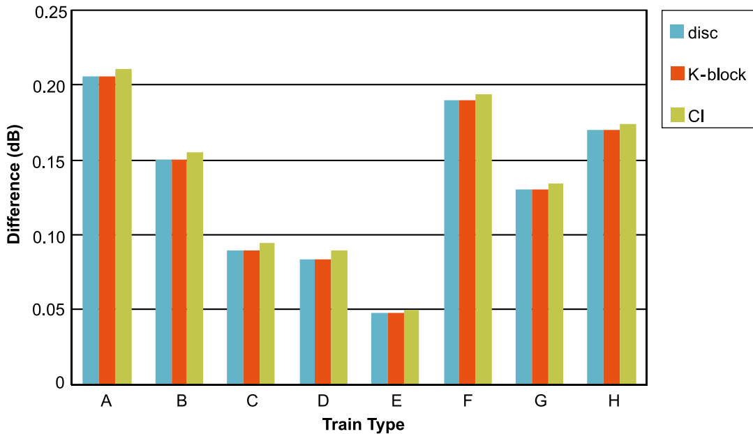
Figure 8. Difference in the equivalent noise level between 920- and 840-mm wheel diameters for accelerating. Notes. disc—disc-braked vehicles, K-block—K-block braked vehicles, CI—cast-iron block-braked vehicles; K-block braked vehicles, CI—cast-iron block-braked vehicles; A—NS Mat64 EMU (Werkspoor/ Düwag/ Waggonfabrik Talbot, The Netherlands); B—NS 1700 (Alsthom, The Netherlands); C—SNCF BB66400 (Vossloh España, Spain); D—SNCF CC72000 (Alsthom-Atlantique, France); E—RENFE (DLoco, Spain); F—NS6400 (MaK/ABB, Germany); G—TKOJ JT 42CWR (EMD, USA); H—DM90 DMU (Dewag/Talbot/SIG, Germany).
