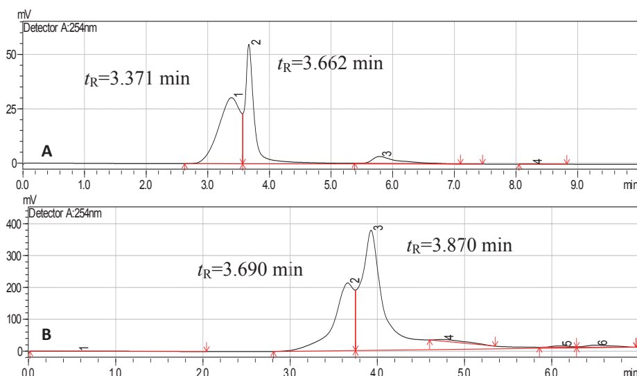
Fig. 6. HPLC chromatogram of FST industrial effluent (A) untreated sample, (B) treated sample, peak 2 for diphenylamine ( t_R=3.690 min), peak 3 for 3-methyldiphenylamine ( t_R=3.870 min) and peaks 4–6 for unknown compounds
