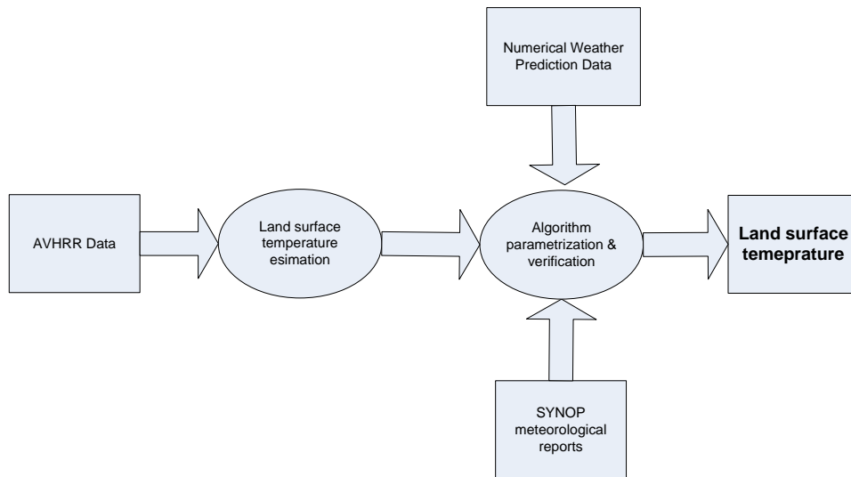
Fig.3. Data sources used in LST estimation and its verification by indirect method.
