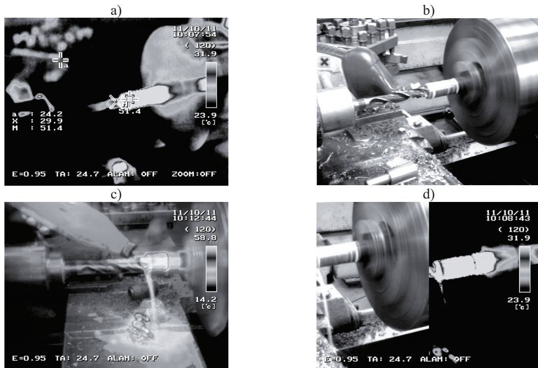
Fig. 4. Displaying images: a) only thermal, b) only visible, c) both parallel, d) mix of both
