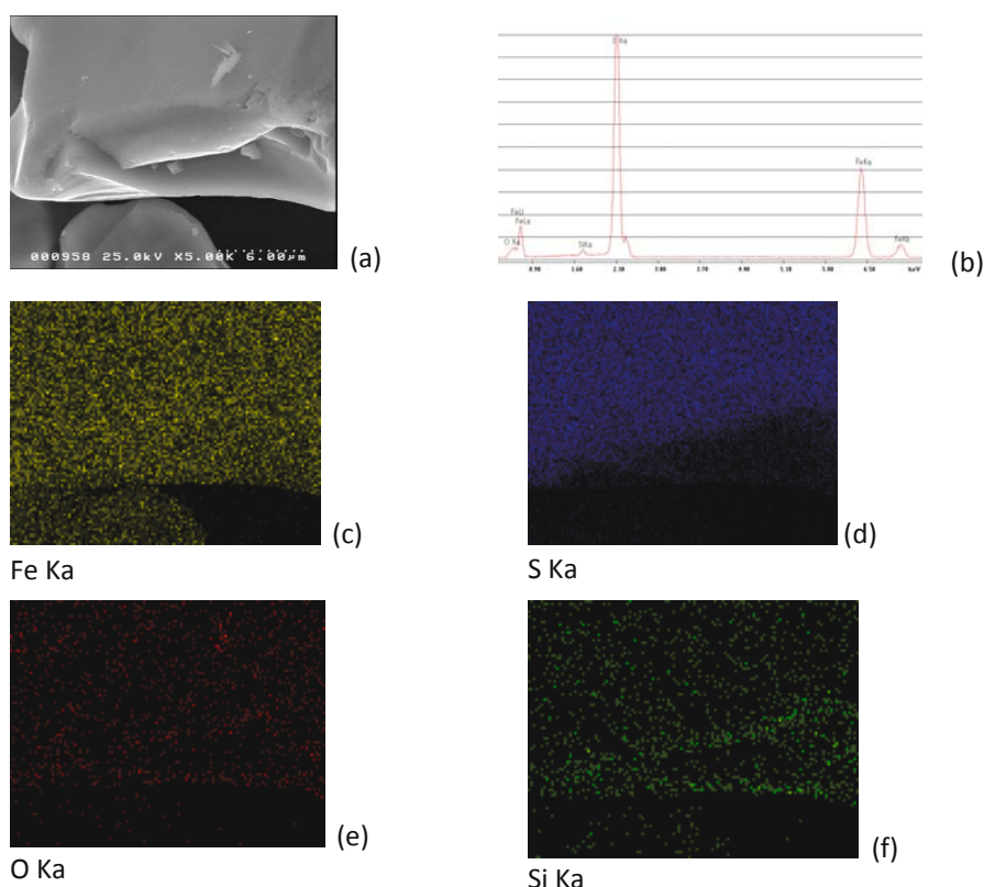
Fig. 2. SEM image and elemental mapping of reacted pyrite samples after 800 h reaction with CB
