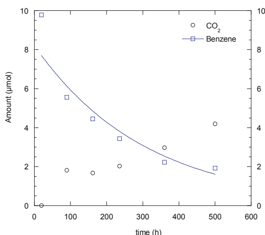
Fig. 6. Degradation profile of benzene and production of CO 2 (pyrite suspension 20 mg/L, 25°C, initial oxygen in equivalent with atmosphere)
