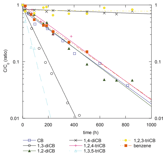
Fig. 9. Degradation profiles of mono-, di- and tri-chlorobenzenes with time in aerobic pyrite suspension (20 m 2 /L), 25°C. Symbols are experimental data. Lines are the calculated curves
