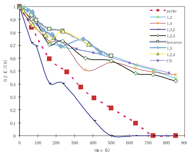
Fig. 10. Oxygen consumption profiles of and aromatic compounds (CBs or benzene) and pyrite with time under aerobic condition
