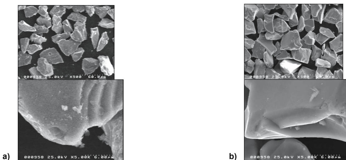
Fig. 1. Secondary electron images of used pyrite mineral: (a) before experiment and (b) after 800h experiment with CB
