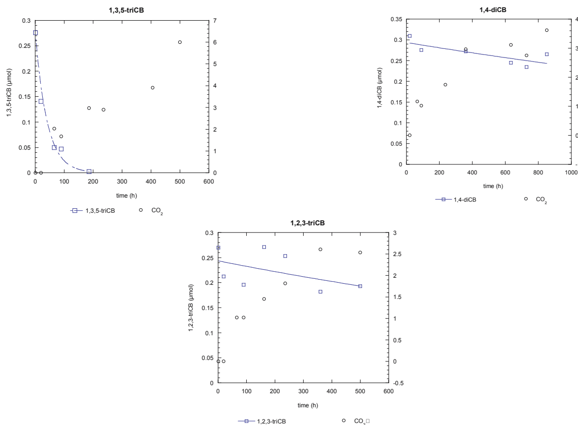
Fig. 8. Degradation profiles of aromatic compounds and CO 2 productions in pyrite suspension (20 m 2 /L), 25°C, initial oxygen in equivalent with atmosphere; a) 135-triCB; b) 14-diCB; c) 123-triCB. Stocks diluted in benzene at concentration of 10 mg/ml for all compounds were used
