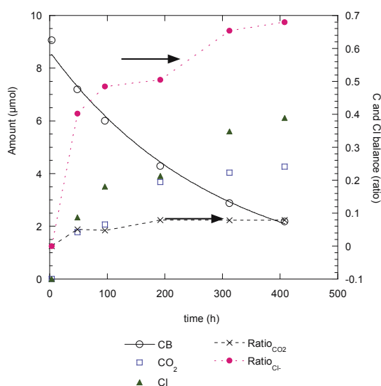
Fig. 4. Degradation of CB, production of chloride and \text{CO}_2 , \text{Ratio}_{\text{Cl}^-} and \text{Ratio}_{\text{CO}_2} (pyrite suspension 20 \text{ m}^2/\text{L} , 25^\circ\text{C} , initial oxygen concentration in equivalent with atmospheric air)
