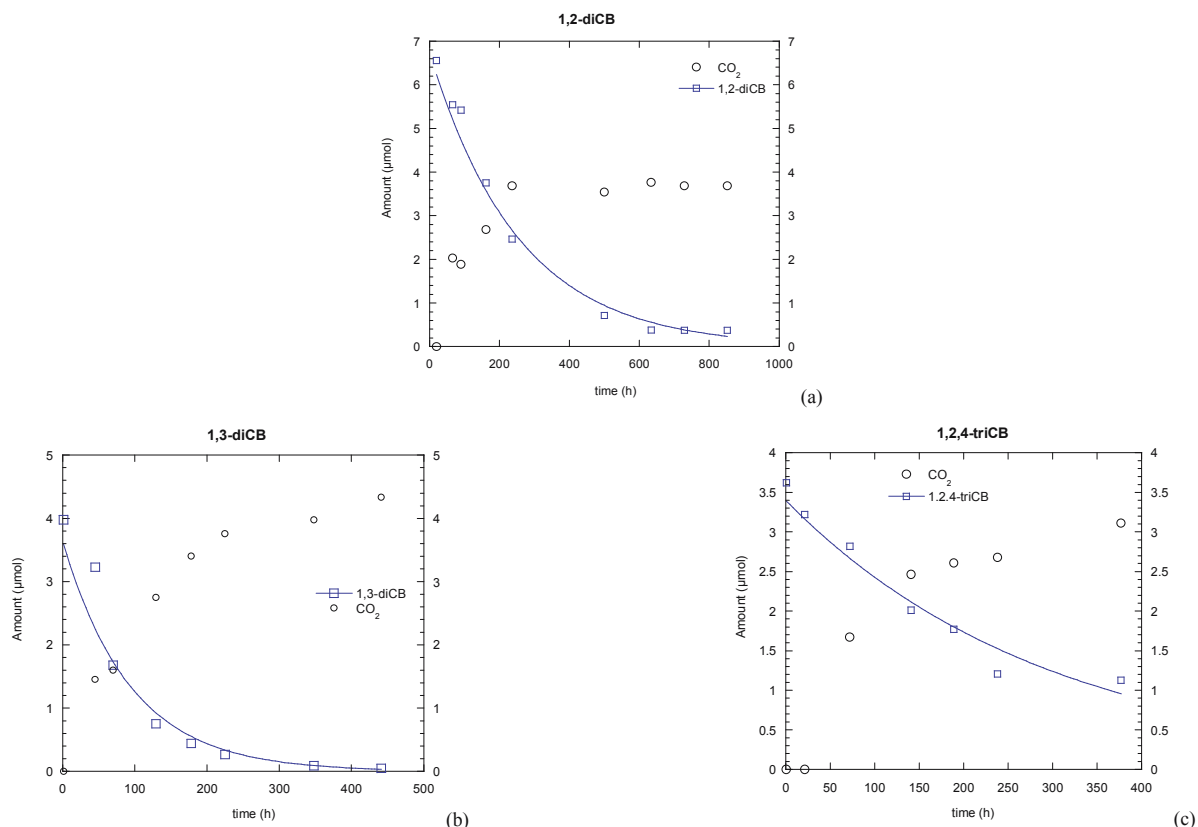
Fig. 7. Degradation profiles of aromatic compounds and CO 2 productions in pyrite suspension (20 m 2 /L), 25°C, initial oxygen in equivalent with atmosphere; a) 12-diCB; b) 13-diCB; c) 124-triCB; Pure stocks of all compounds were used
