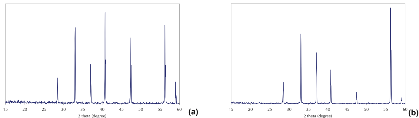
Fig. 3. XRD measurements of unreacted (above) and reacted pyrite (below)
