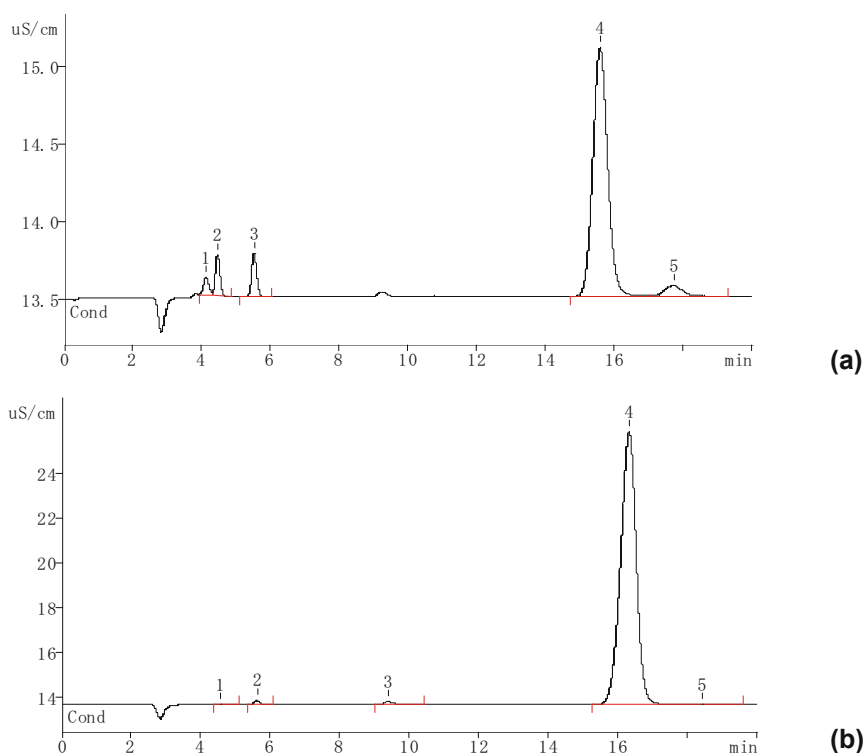
Fig. 5. Ion chromatography spectra. a) CB in pyrite suspension (Peak names: 1. Acetic acid, 2. Pyruvic acid and/or formic acid, 3. Chloride ion, 4. Sulfate ion, 5. Oxalic acid); b) Pyrite suspension blank (Peak name: 2. Chloride ion, 4. Sulfate ion)
