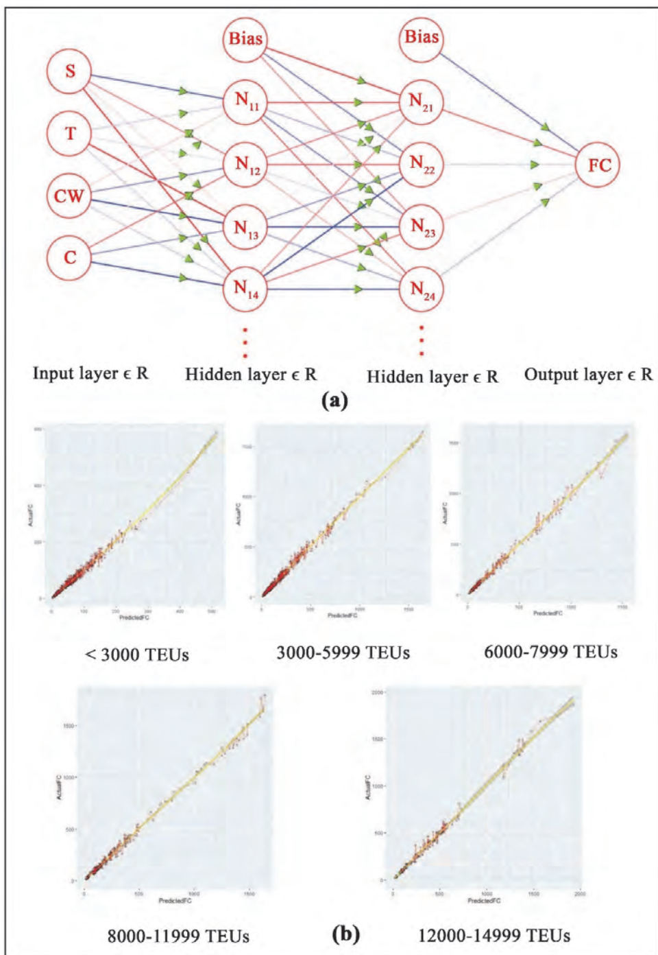
Fig. 6. (a) – ANN model with 2 hidden layers; (b) – Actual and estimated fuel consumption [169]
