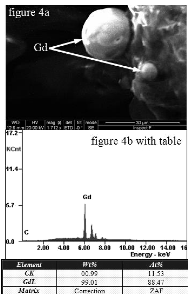
Fig. 4. The results of the experiment: Fig. 4a – SEM image of Gd microparticles in paraffin after seven months after creation; Fig. 4b – EDX analysis performed for the gadolinium particle with a table of compositional analysis of Gd. The spectrum shows mainly gadolinium with a small doping of carbon without any trace of oxygen peak, which should be located between carbon and gadolinium peaks, at energy of 0.5 [eV]. All 4 peaks on right side of gadolinium peak belong also to Gd.
