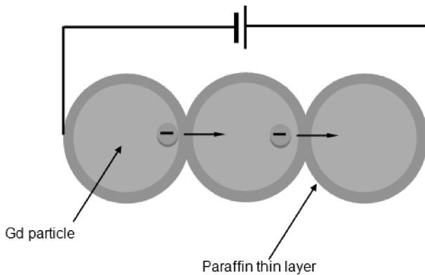
Fig. 2. Scheme of electron conduction Gd – paraffin composite material. Particles of gadolinium are close to each other and covered by thin film of paraffin which allows diffusion of electron from one Gd particle to another.
