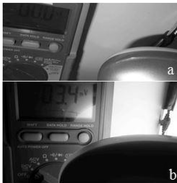
Fig. 1. Gd-paraffin sample: a) Gd-paraffin sample in an open circuit configuration held by steel electrodes; a fluorescent lamp switched of – voltage: 0 [V]; b) Gd-paraffin sample illuminated by the fluorescent lamp – voltage: 3.4 [mV].
