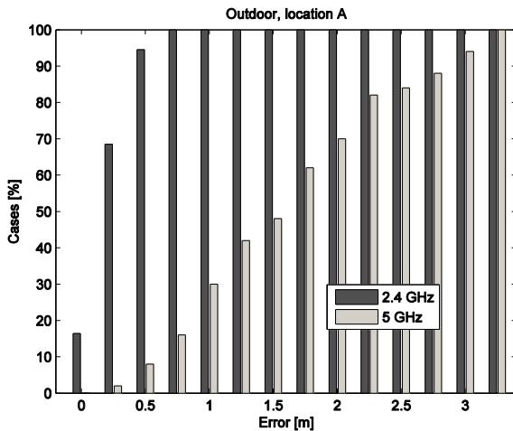
Fig.16. Cumulative histogram of positioning error for location A.
