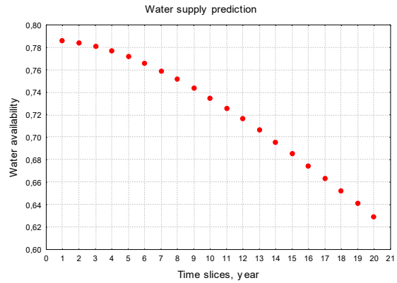
Fig. 7. Water availability as a function of time for meshed network; source: own study
