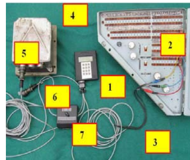
Fig. 9. A DIA-Mi24 connected to Mi24 helicopter's electrical infrastructure sub-assemblies 1 – DIA-Mi24 tester, 2 – AC switchboard of the Mi-24 helicopter, 3 – three-phase electrical bundle connecting the electrical circuits of the helicopter 3x36 V, 400 Hz with the DIA Mi24 tester (channel A+B), 4 – voltage regulator of the on-board generator no. 1 (tie-in location of the diagnostic tester), 5 – reception connector for the pilot exciter voltage signal from the voltage regulator of generator no. 1, 6 – reception connector for the pilot exciter voltage signal from the voltage regulator of generator no. 2, 7 – pilot exciter measurement chain switch (pilot exciter no. 1 – pilot exciter no. 2)
