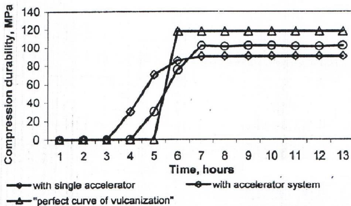
Figure 2. Kinetic curves of compression durability gainig. 1 – with single accelerator, 2 – with accelerator system, 3 – “perfect curve” of vulcanization.
