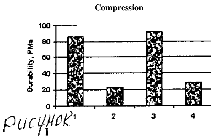
Figure 1. TValues of \sigma_{com} and \sigma_b of RubCon for various rubbers. 1- PotyoiIR, 2-PBNR, 3- Ricon 130R, 4-SKDN-NR.
