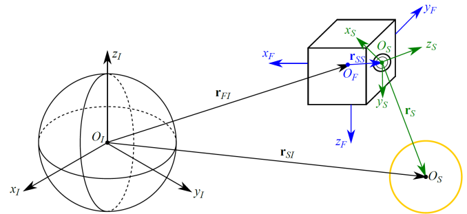
Fig. 2. Sun sensor direction vectors
