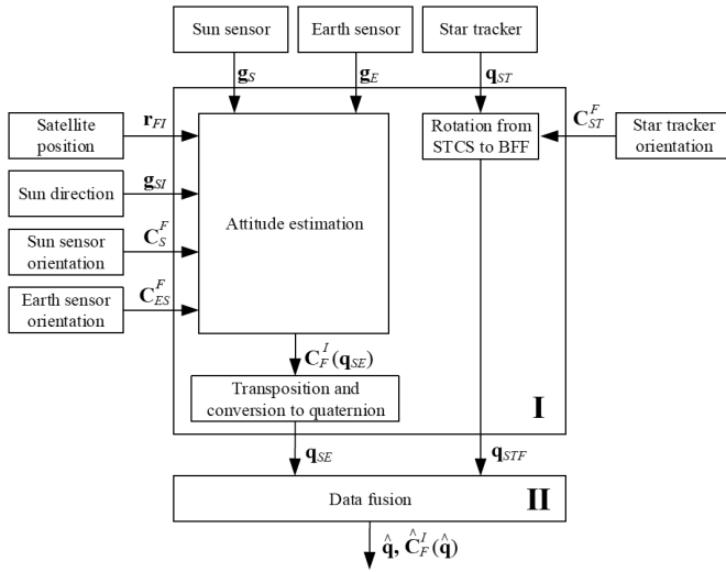
Fig. 1. Attitude calculation methodology
