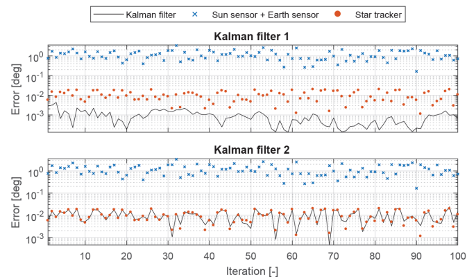
Fig. 8. Kalman filtering results
