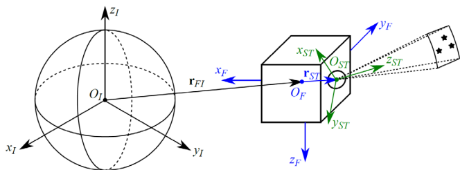
Fig. 4. Star tracker direction vectors
