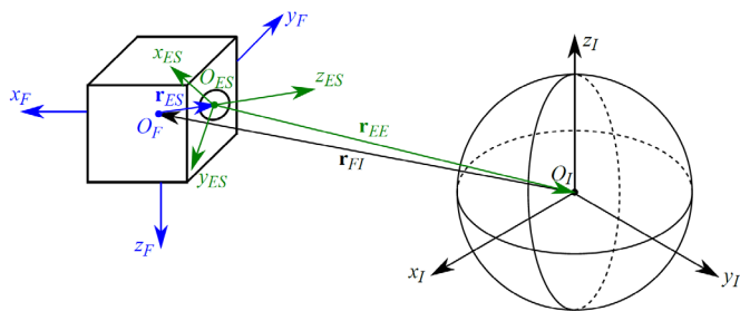
Fig. 3. Earth sensor direction vectors
