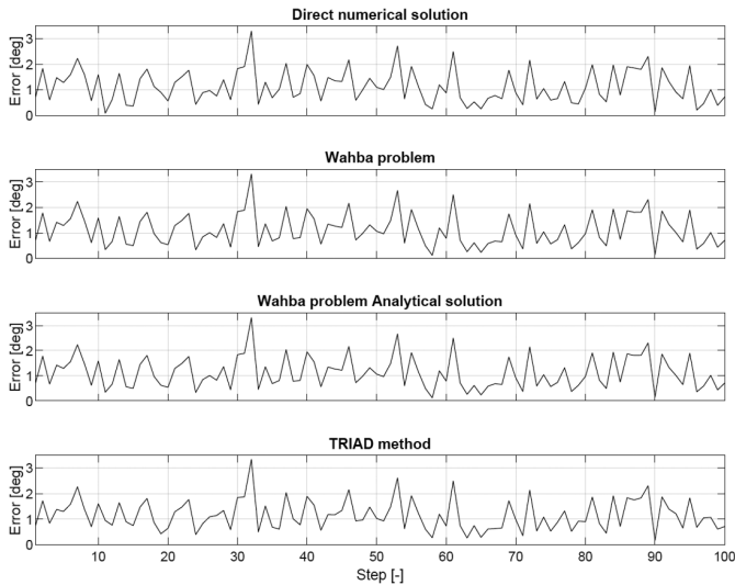
Fig. 7. Errors for sun and earth sensor integration
