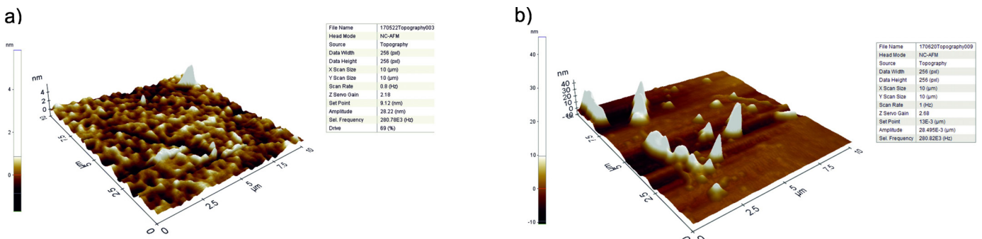
Fig. 2. Surface geometry of the EOS CoCr SP2: a) initial state, b) with ZrO 2 layer
