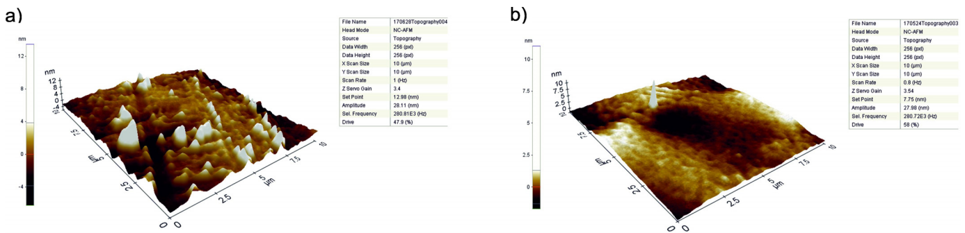
Fig. 1. Surface geometry of the Realloy C: a) initial state, b) with ZrO 2 layer
