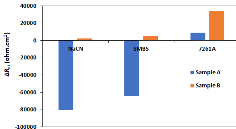
Fig. 8. The differences in R_{ct} values of "Dep" and the experiments conducted with NaCN:KAX, SMBS:KAX and 7261A:KAX
