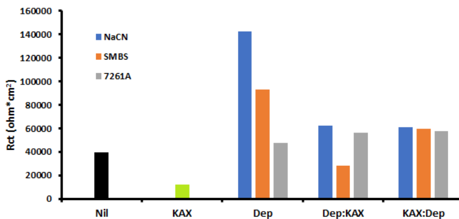
Fig. 4. Coating resistance ( R_{ct} ) of Sample A under different experimental conditions at pH 9.2, 100 mV polarization potential. (Nil: absence of collector and depressants; KAX: collector; Dep:depressant; Dep:KAX depressant addition prior to KAX, and KAX:Dep KAX addition prior to depressant)
