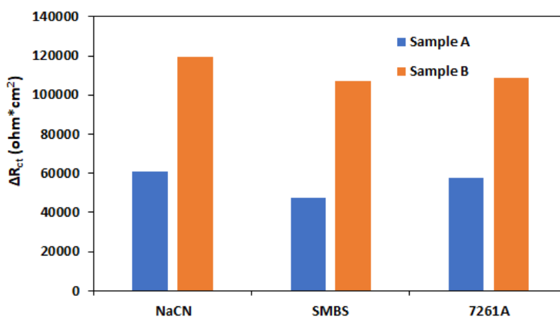
Fig. 9. The differences in R_{ct} values of "KAX" and the experiments conducted with KAX:NaCN, KAX:SMBS and KAX:7261A
