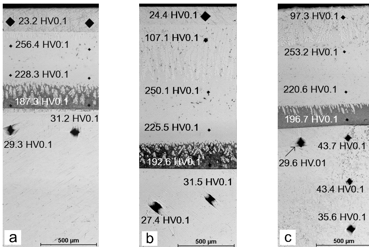
Fig. 4. Indentations in the Al-alloyed layers and the magnesium substrate formed under various casting conditions: (a) variant 1, (b) variant 2, (c) variant 3
