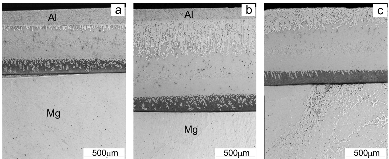
Fig. 1. Microstructures of the surface layer formed by the reaction between the molten magnesium and the aluminium insert: (a) variant 1, (b) variant 2, and (c) variant 3
