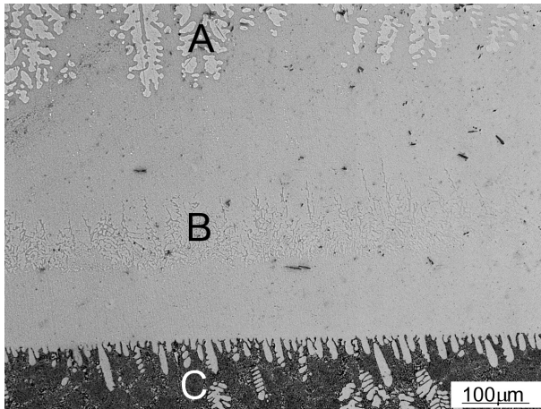
Fig. 2. Enlarged OM image of the layer microstructure
