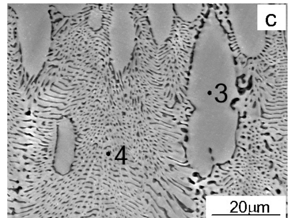
Fig. 3. SEM images showing details of the layer microstructure: (a) zone A, (b) zone B, (c) zone C
