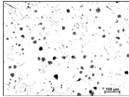
Fig. 7. Graphite precipitates in cast iron containing 5.18% Al and 5.24% Si (melt IV), non-etched micro-section, magn. 100×
