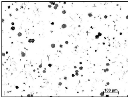
Fig. 11. Graphite precipitates in cast iron containing 5.35% Al and 5.30% Si (melt VI), non-etched micro-section, magn. 100×
