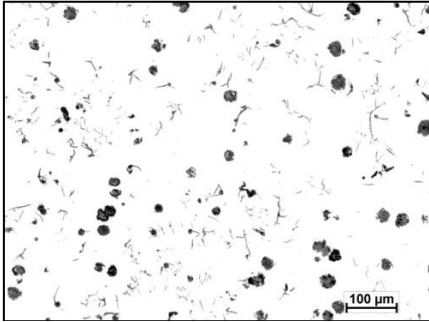
Fig. 5. Graphite precipitates in cast iron containing 6.02% Al and 4.97% Si (melt III), non-etched micro-section, magn. 100×
