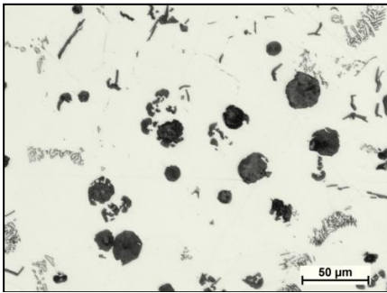
Fig. 4. The microstructure of cast iron containing 5.13% Al and 4.98% Si (melt II), etched micro-section, magn. 300×
