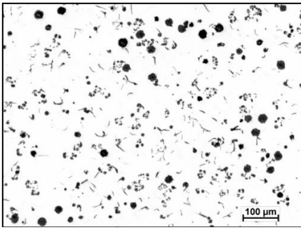
Fig. 3. Graphite precipitates in cast iron containing 5.13% Al and 4.98% Si (melt II), non-etched micro-section, magn. 100×
