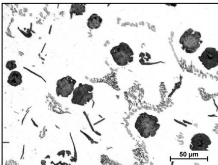
Fig. 6. The microstructure of cast iron containing 6.02% Al and 4.97% Si (melt III), etched micro-section, magn. 300×
