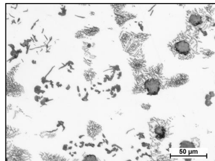
Fig. 2. The microstructure of cast iron containing 5.64% Al and 4.50% Si (melt I), etched micro-section, magn. 300×
