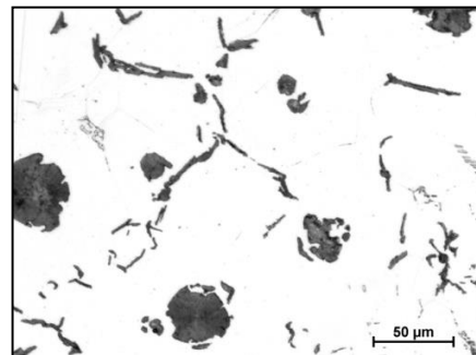
Fig. 10. The microstructure of cast iron containing 5.30% Al and 5.28% Si (melt V), etched micro-section, magn. 300×
