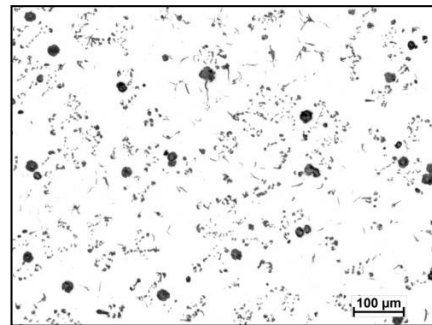
Fig. 1. Graphite precipitates in cast iron containing 5.64% Al and 4.50% Si (melt I), non-etched micro-section, magn. 100×
