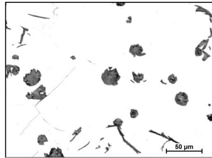
Fig. 8. The microstructure of cast iron containing 5.18% Al and 5.24% Si (melt IV), etched micro-section, magn. 300×
