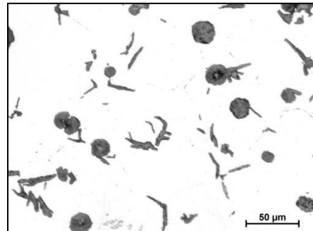
Fig. 12. The microstructure of cast iron containing 5.35% Al and 5.30% Si (melt VI), etched micro-section, magn. 300×
