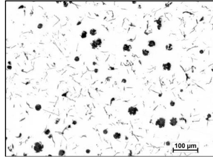
Fig. 9. Graphite precipitates in cast iron containing 5.30% Al and 5.28% Si (melt V), non-etched micro-section, magn. 100×
