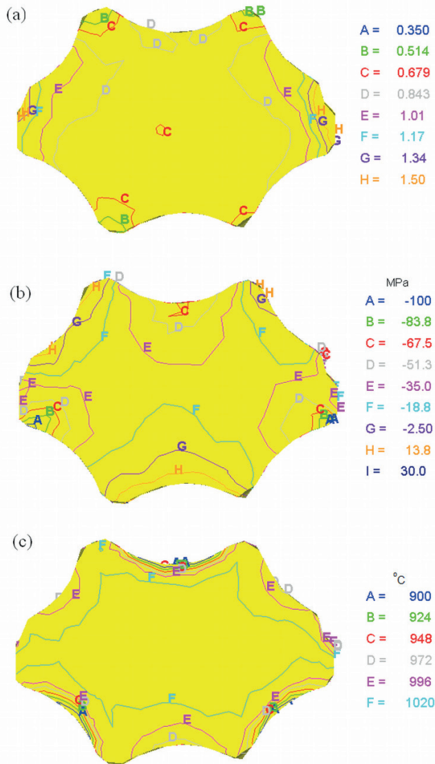
Fig. 5. Distribution of effective strain (a), mean stress (b) and temperature (c) on the specimen cross-sectional surface after cogging process in special tri-radial anvils. True strain \epsilon_h = 0.70
