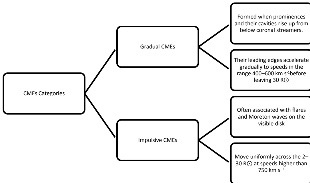
Figure 1. Categories of Coronal Mass Ejections (CMEs).
