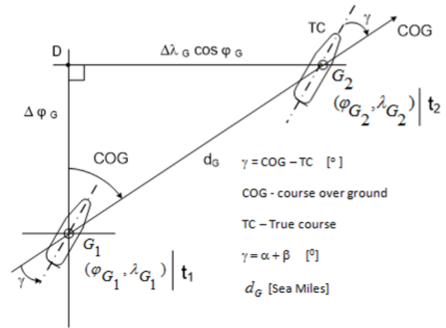
Figure 3. Setting of two fixes G_1 and G_2 to determine course over ground
