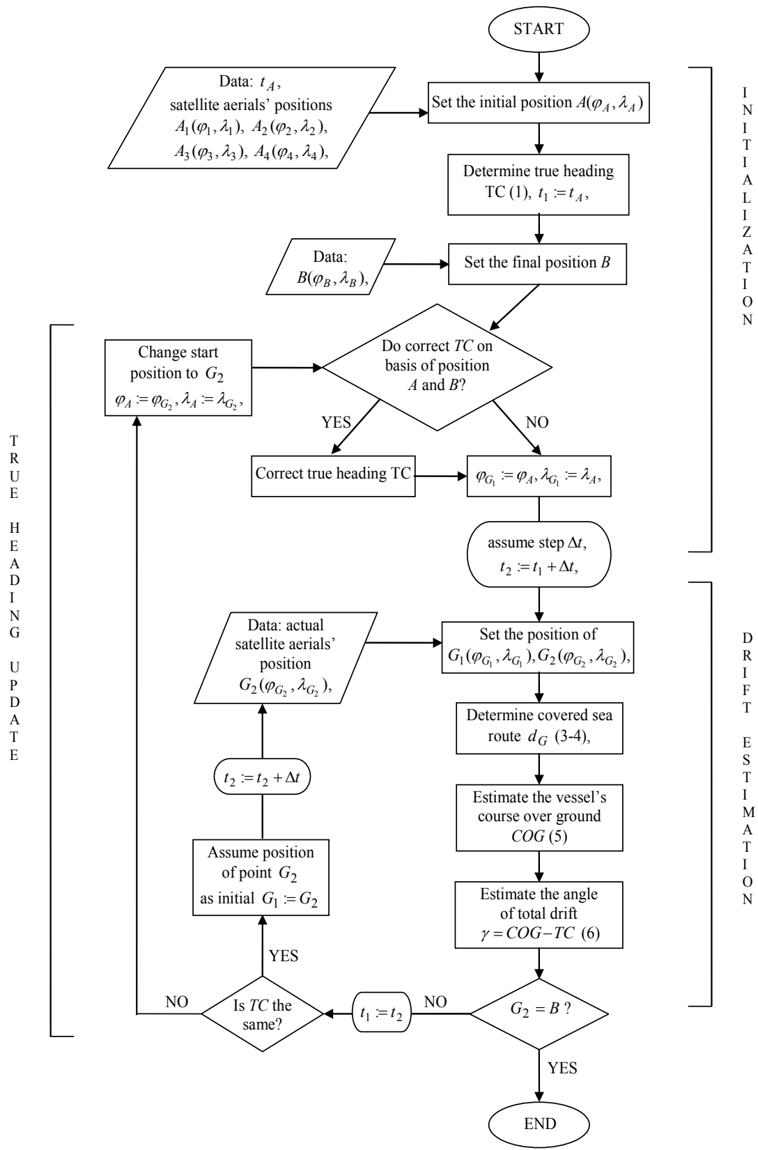
Figure 4. Block diagram for true heading and angle of vessel's total drift calculation
