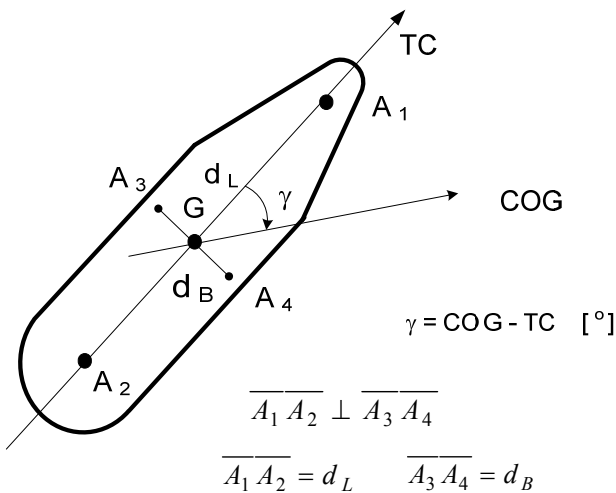
Figure 2. Two bases on board using four GPS receivers for COG determination
