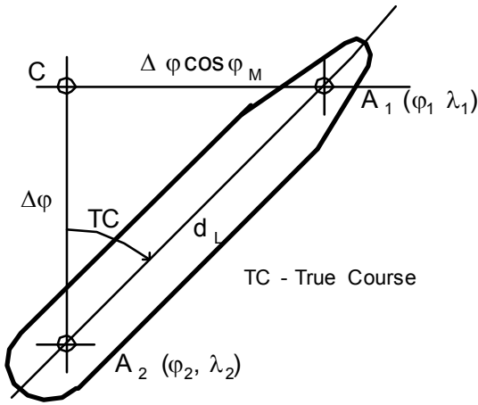
Figure 1. Base line on board the ship using two GPS receivers for true course determination
