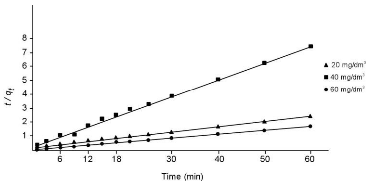
Fig. 7. Pseudo-second-order plots for adsorption of rhodamine B onto natural diatomite
