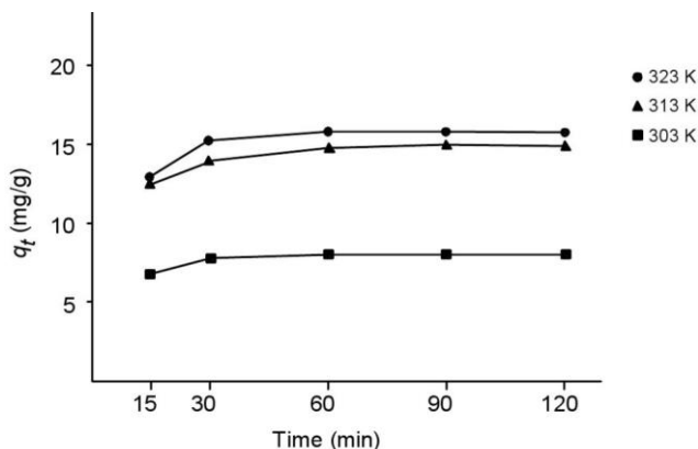
Fig. 3. Effect of temperature on adsorption of Rh-B onto natural diatomite
