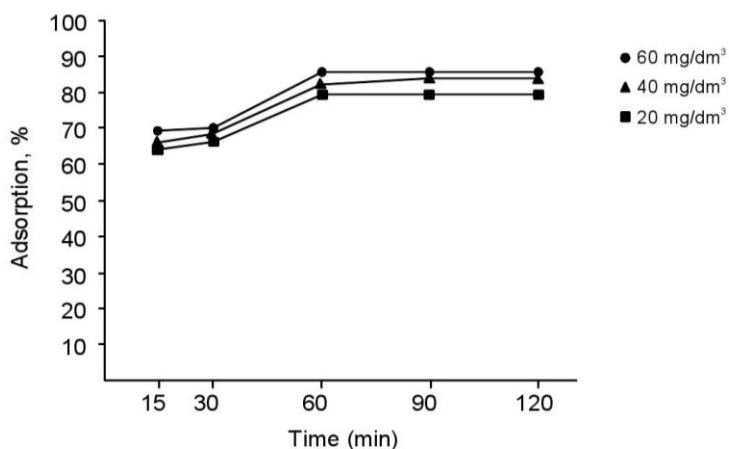
Fig. 2. Effect of contact time and initial dye concentration on dye adsorption. Natural diatomite dose 1 \text{ g/dm}^3 (pH 8 \pm 0.2 at 323 K)
