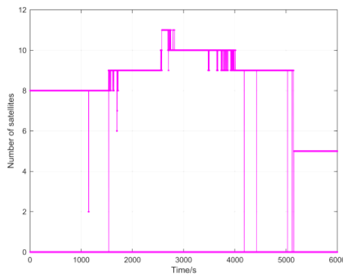
Fig. 4. The number of BeiDou satellites
