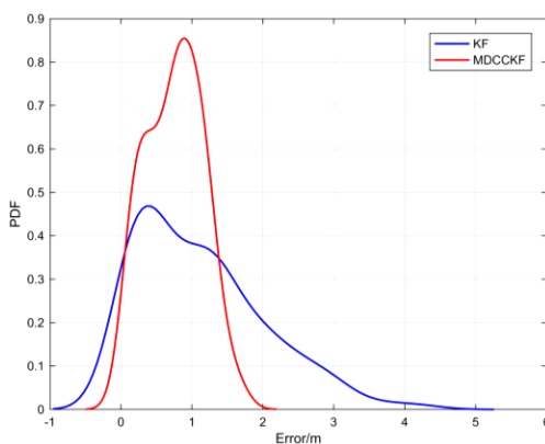
Fig. 10. The PDF of positioning error ( \alpha = 1.25 )
