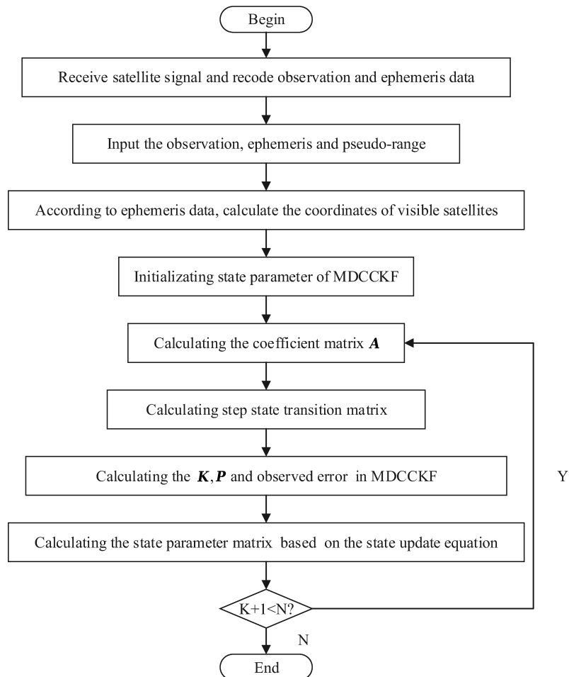
Fig. 1. The flowchart of MDCCKF positioning algorithm
