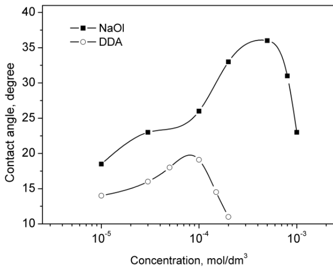
Fig. 4. Contact angles at FA surface depending on the NaOI and DDA concentrations at pH 9.5
