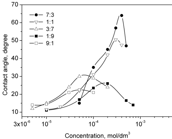
Fig. 5. Contact angles at FA surface depending on concentration and molar ratio of NaOI-DDA mixtures at pH 9.5
