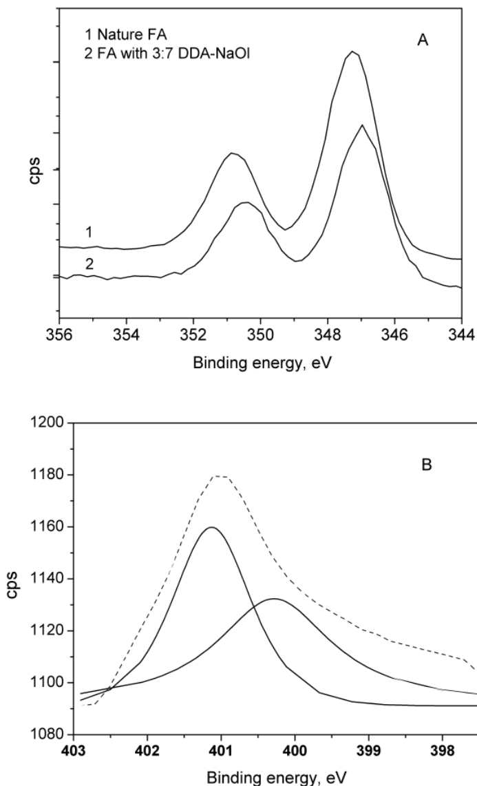
Fig. 6. XPS results of Ca2p peaks (A) and N1s peaks (B) of FA treated with the 3:7 DDA-NaOI mixture
