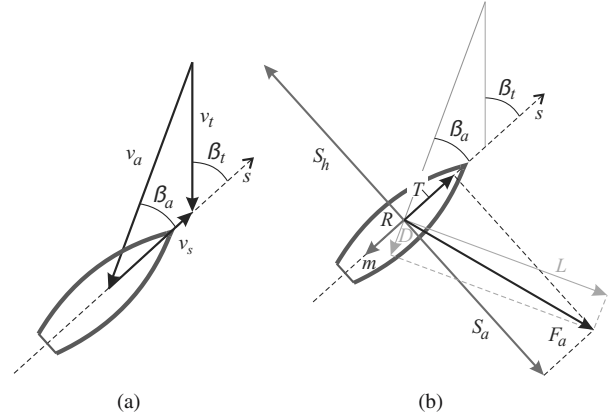
Fig. B1. Sailboat (sailing upwind) model used in Example 2. Here, \beta_t : true wind angle, \beta_a : apparent wind angle, s : (current) sailing direction, v_t : true wind velocity, v_a : apparent wind velocity, v_s : current sailboat velocity, F_a : aerodynamic force, L : lift (the aerodynamic force component perpendicular to the wind direction), D : drag (the aerodynamic force component in the direction of the wind), T : thrust, S_a : side force, S_h : hydrodynamic side force, R : total (i.e., hydrodynamic plus aerodynamic) resistance. Velocities (a), forces (b).
