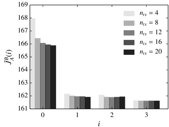
Fig. 14. Values of the performance measure ( \bar{J}_A^B ) for subsequent refinements of five different multi-splines (defined respectively by n_{ts} = 4, 8, \dots, 20 ). In all instances, n_r = 16 and n_c = 32 .
