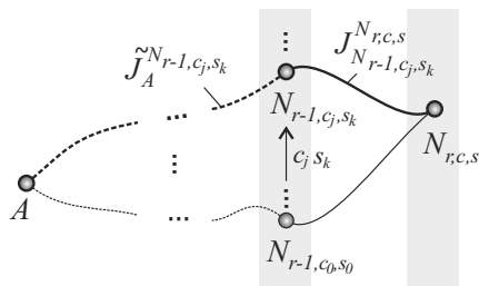
Fig. 6. Principle of optimality in dynamic programming: optimal path (trajectory) from point A to point N_{r,c,s} ( G_{ex} node); graphical representation of Eqn. (16) (with the notation J_{from}^0 and \bar{J} representing the optimal J ).
