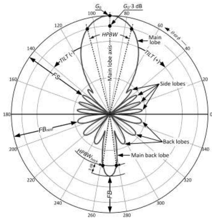
Fig. 3. Modelled radiation pattern
