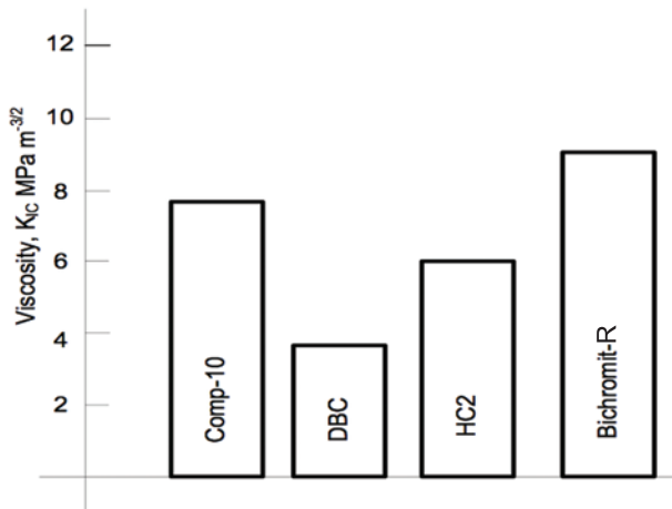
Fig. 3. Fracture toughness diagrams of several cutting tool materials
