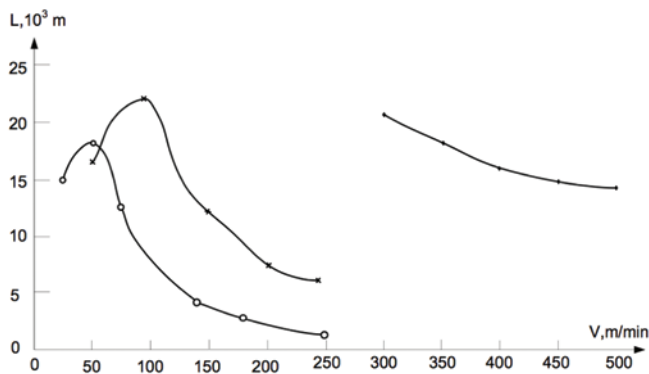
Fig. 5. Cutting speed influence on the wear of a cutting tool h_3 = 0.4\text{ mm} , during turning of steel 30X1CA (HRC 58-62) at f = 0.075\text{ mm/rev} , and p = 0.2\text{ mm} , -o- Silinite-P; -X- BOK-71; -□- Bichromit-R
