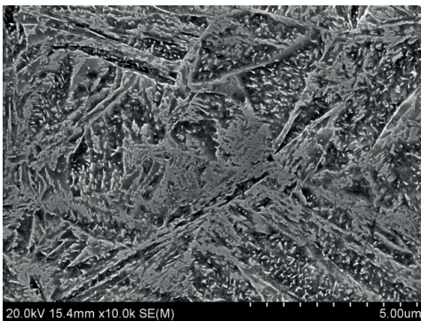
Fig. 3. Cross-sectional microstructure of screw after Process no. 2: a) subsurface below zinc layer; (b–d) area in core of screw; SEM; etched with 2% nital
