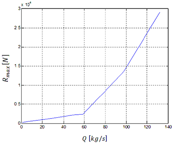
Fig. 12. Maximum force transmitted to the foundation as the efficiency function
