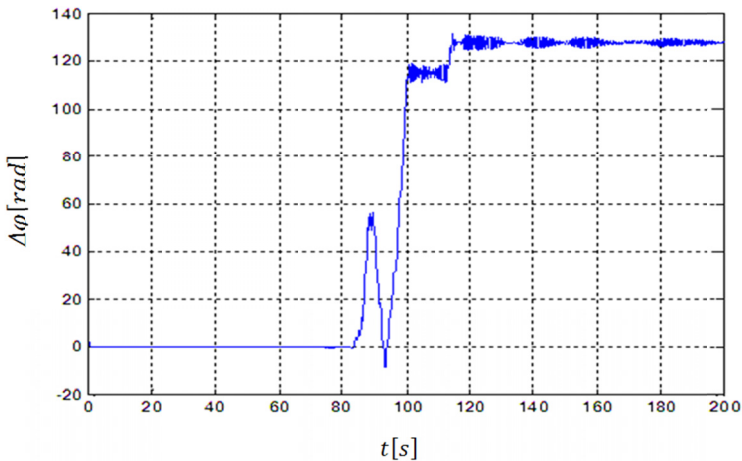
Fig. 14. Difference of angular displacements of engines 1 and 2 at coasting
