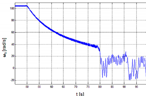
Fig. 15. Effect of loosing the vibrator angular frequency in the circum-resonant range
