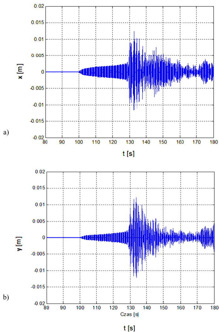
Fig. 16. Free coasting of the machine (the drive was switched off in the 100-th second of the simulation): a) Horizontal displacement of the body, b) Vertical displacement of the body
