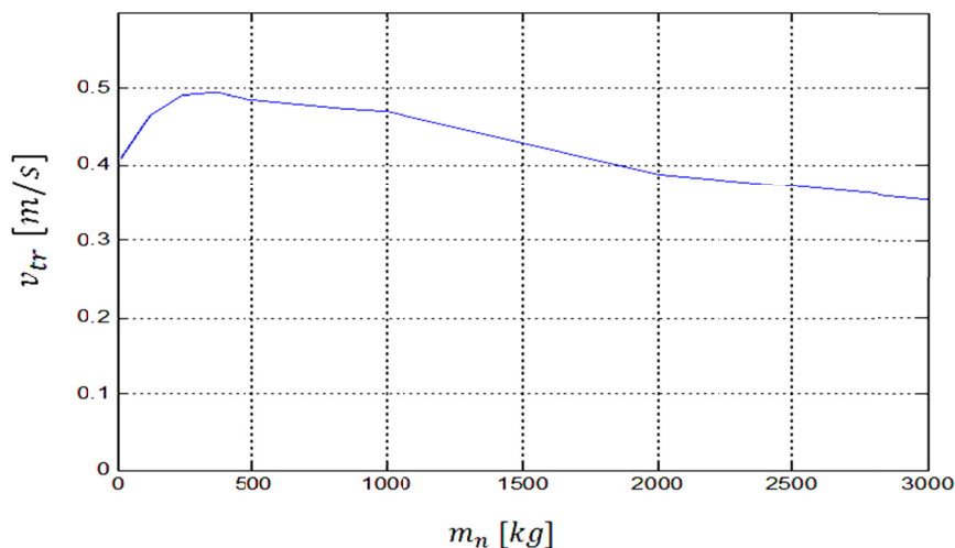
Fig. 10. Dependence of the average transport velocity v_{tr} (averaged in layers) of the conveyor loaded with the feed m_n
