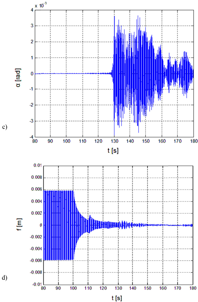
Fig. 16. Free coasting of the machine (the drive was switched off in the 100-th second of the simulation): c) Angular displacement of the body, d) Relative displacement of the trough
