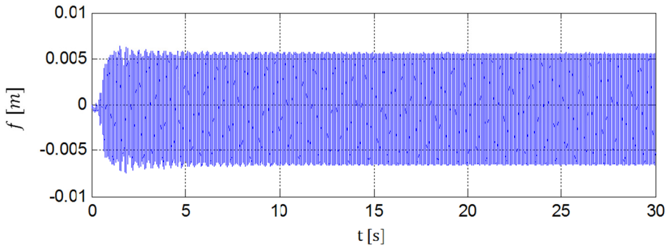
Fig. 9. Relative displacement f of the trough versus the body, as a time function
