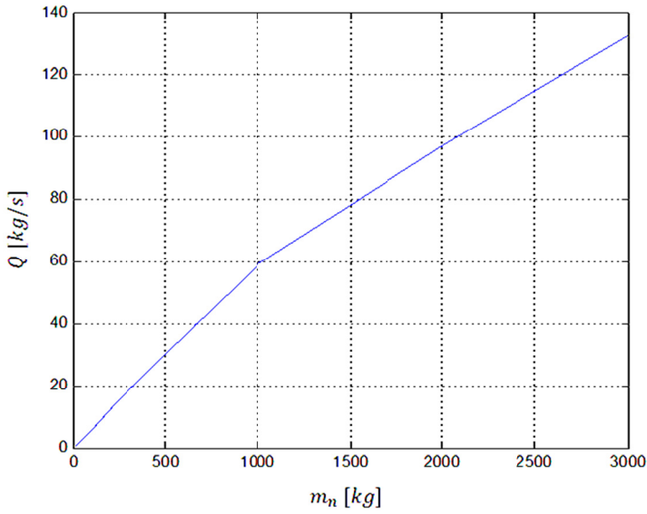
Fig. 11. Conveyor efficiency Q as a function of the feed mass being on the conveyor trough m_n
