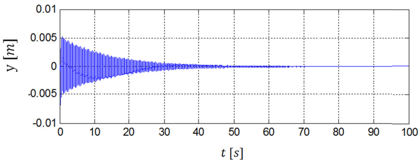
Fig. 4. Vertical displacement of the conveyor body mass as a time function
