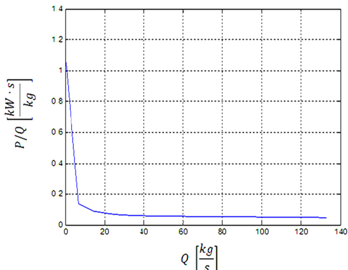
Fig. 13. Ratio of the power demand to the efficiency as the efficiency function obtained on the basis of simulation
