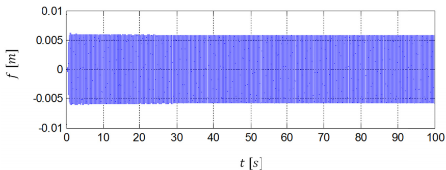
Fig. 5. Displacement of the trough f versus the body as a time function
