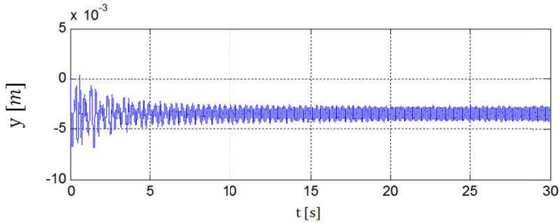
Fig. 8. Vertical displacement y as a time function
