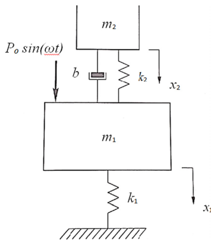
Fig. 1. Scheme of operation of antiresonance vibratory conveyors
