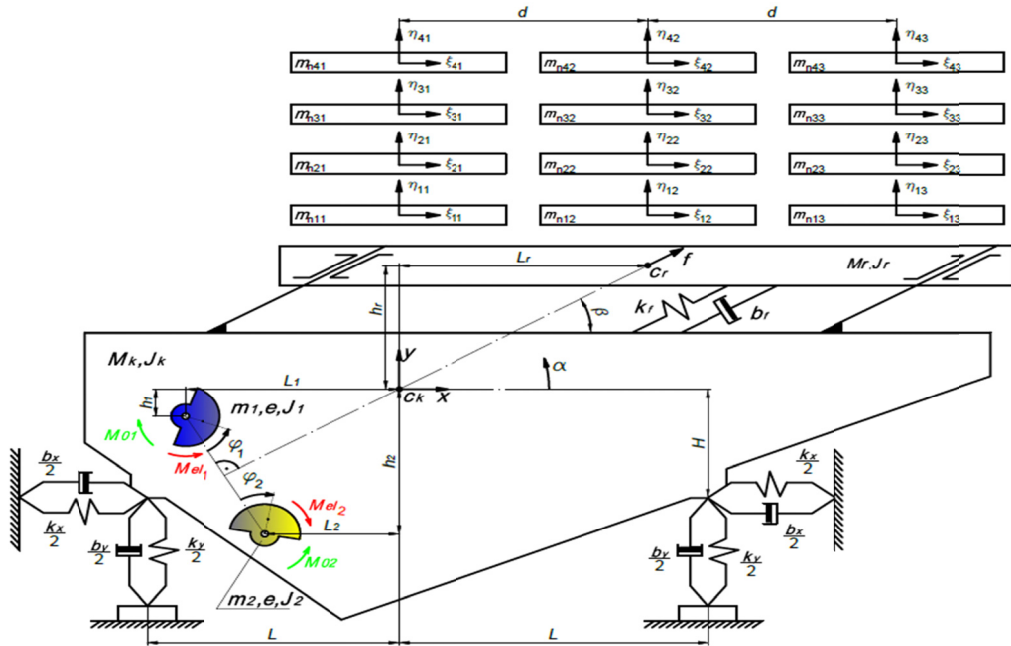
Fig. 3. Model of the vibratory conveyor, where f – relative displacement M_r in relation to M_k
