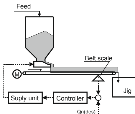
Fig. 13. System of the volumetric flow stabilization to a jig
