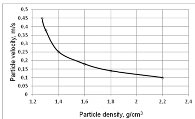
Fig. 9. Velocity of a particle as a function of a particle density
