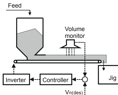
Fig. 14. System of the feed tonnage control
