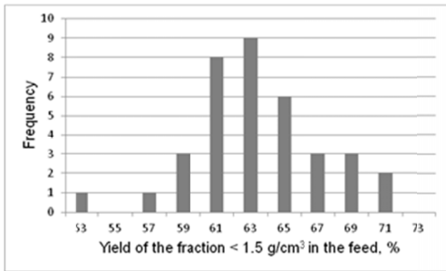
Fig. 8a. Yield of the density fraction <1.5 \text{ g/cm}^3
