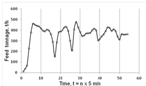
Fig. 4. An example of variations of the feed flow to a jig
