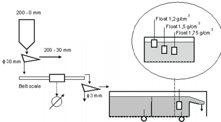
Fig. 10. Technological system (Kowol, 2011)
