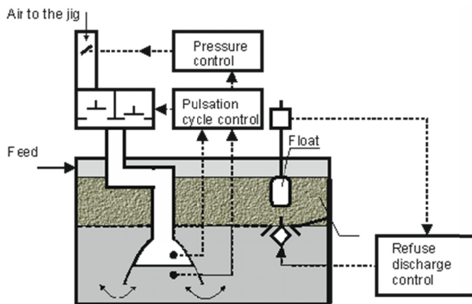
Fig. 1. Block scheme of the control of a pulsation cycle and refuse discharge
