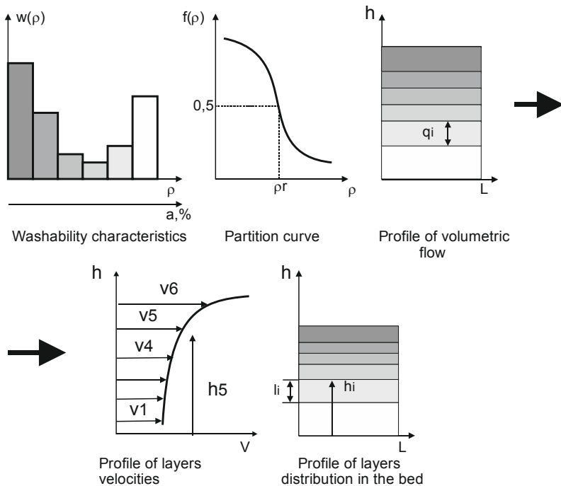
Fig. 3. Density layers forming in the bed
