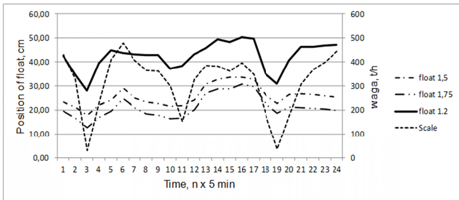
Fig. 11. Position of density layers in the jig's bed and changes in tonnage of the feed
