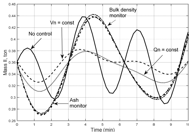
Fig. 17. Changes in the material mass in the bed (II compartment) produced by changes in the feed parameters and errors of measurement
