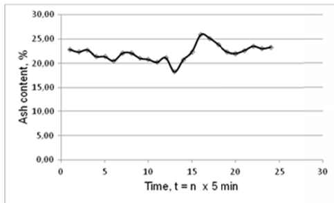
Fig. 6. An example of ash content variations in a jig feed
