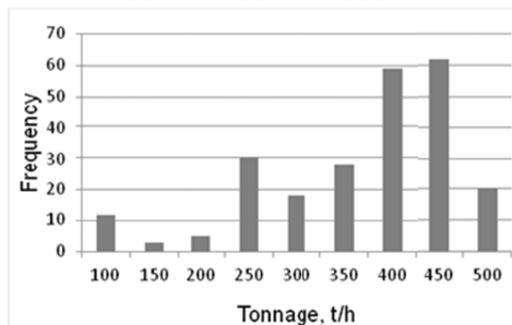
Fig. 5. A distribution of the feed flow
