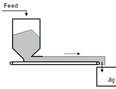
Fig. 12. Technological system of a bunker and a jig
