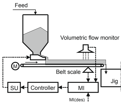
Fig. 15. Control system with the measurement of bulk density
