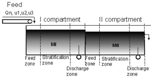
Fig. 2. Zones of the feed, stratification and product discharge in a jig
