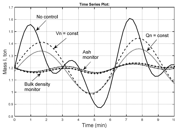
Fig. 16. Changes in the material mass in the bed (I compartment) produced by changes in the feed parameters and errors of measurement
