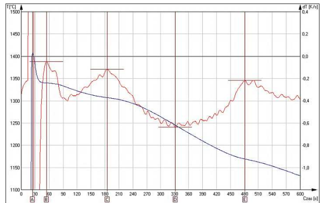
Fig. 3. ATD graph for IN-713C (master heat 3V6577/T5)
